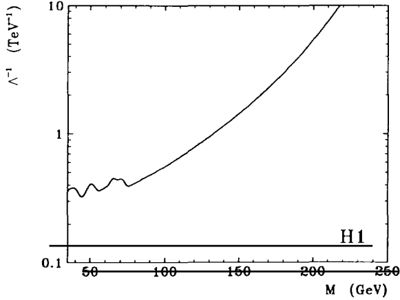
Fig. 3. Rejection limits at the 95% CL for the inverse of the scale parameter \Lambda versus M for e_8 leptogluons. Values above the curve are excluded.
