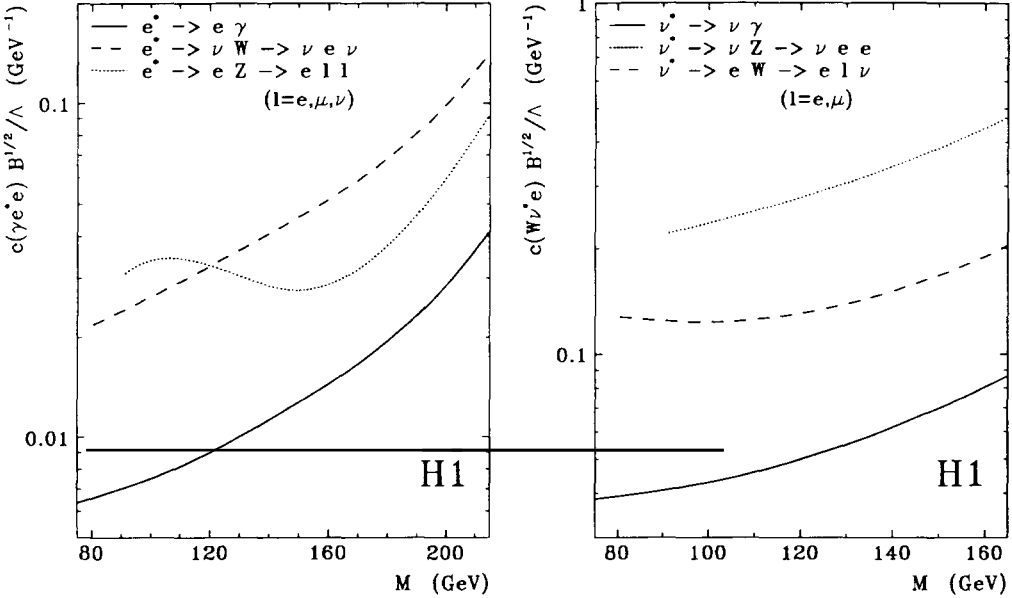
Fig. 4. Rejection limits with a CL of 95% for the e^* and the \nu^* . Regions above the curves are excluded. For masses above 120 GeV the main contribution in the decay channel e^* \rightarrow eZ stems from the decay Z \rightarrow \nu\nu . For lower masses the trigger efficiency for this channel decreases and in that region the limits are determined by the decays Z \rightarrow ee(\mu\mu) .
