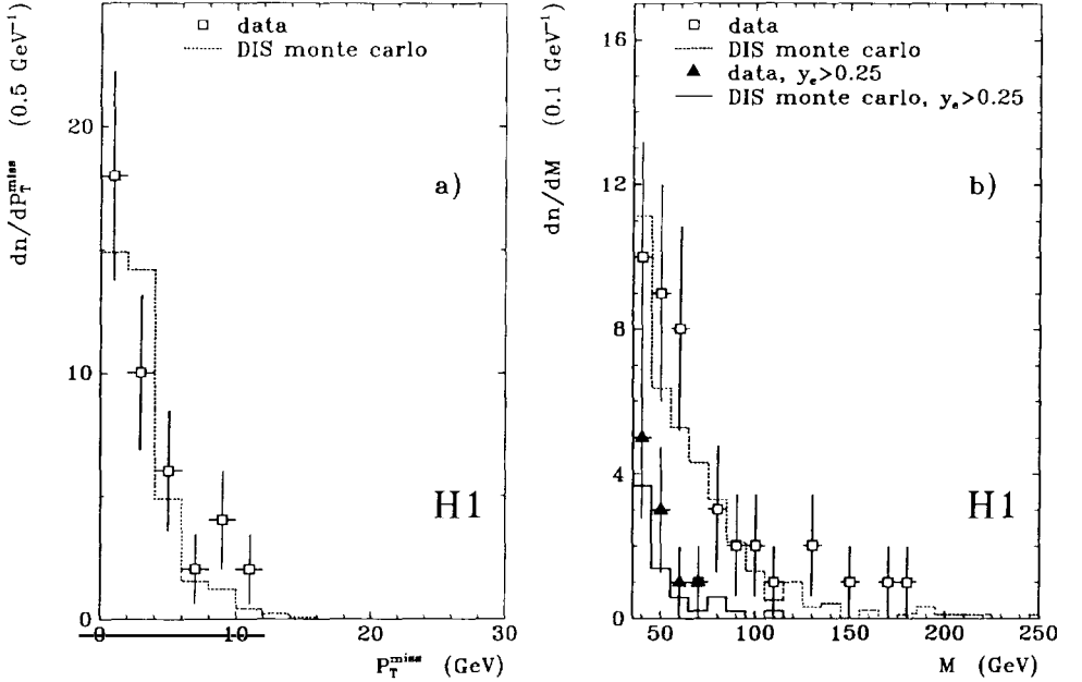
Fig. 1. P_T^{\text{miss}} distribution (a) and mass spectrum (b) for M = \sqrt{x_e s} > 35 \text{ GeV} before (open points) and after (closed points) the final kinematical cut on y_e . The histogram curves show the absolute prediction of a DIS Monte Carlo simulation based on DJANGO before (dashed) and after the (solid) kinematical cut.
