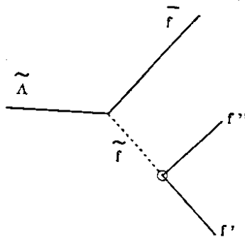
Fig. 4. R decay of the LSP, assumed to be the lightest neutralino \tilde{\Lambda} , where f denotes either quark or lepton.
