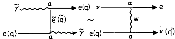
Fig. 2. Comparison of photino and neutrino interaction rates with ordinary matter, i.e. electrons and quarks.
