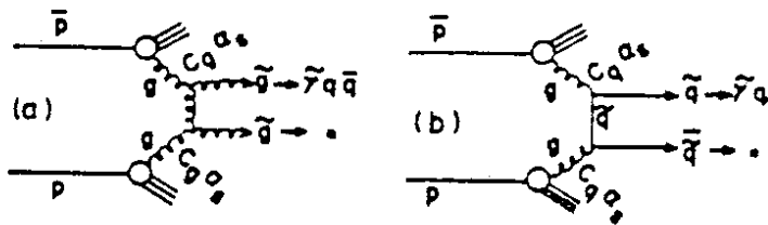
Fig. 3. Strong production of gluino and squark pair, followed by their decay into the LSP ( \tilde{\gamma} ).
