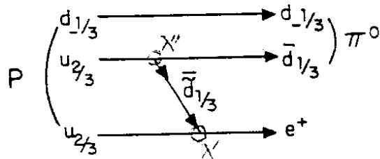
Fig. 1. Proton decay via squark exchange in R SUSY model.
