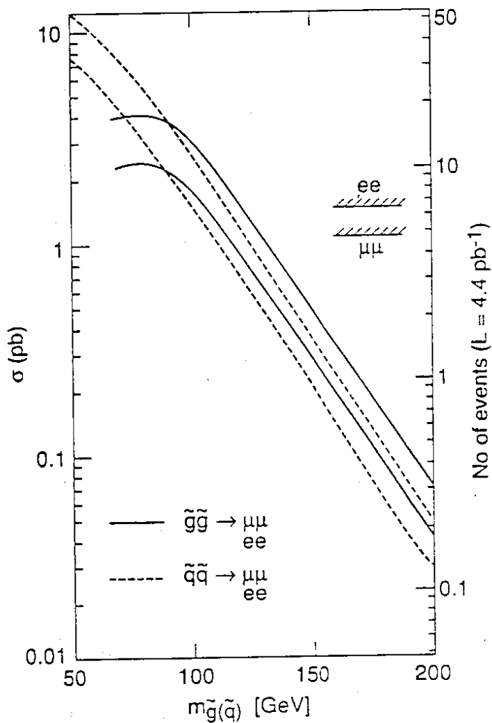
Fig. 6. The visible dimuon and dielectron cross-sections, following the kinematic cuts of Table 1, are shown as functions of gluino (squark) mass. The right hand scale shows the expected number of events for the CDF luminosity of 4.4 \text{ pb}^{-1} . The 95% CL limits shown correspond to 1 dimuon and 2 dielectron events remaining in the CDF data after these kinematic cuts.
