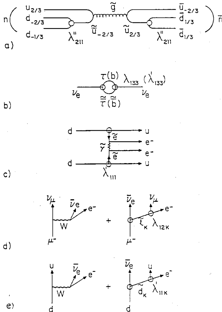
Fig. 5. The R SUSY model contribution to (a) neutron-antineutron oscillation, (b) \nu_e mass, (c) neutrinoless double beta decay, (d) muon beta decay and (e) neutron beta decay.
