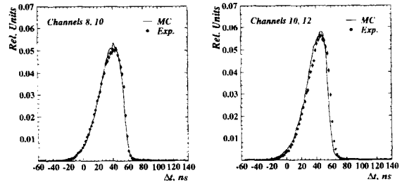
Fig. 13. Distribution of light arrival time differences \Delta t_{i,j} = t_j - t_i for different channel combinations. Points are experimental data, MC results are given by the solid line.
