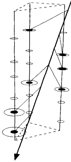
Fig. 15. Single muon event recorded with NT-36. Hit channels are in black. The thick line gives the reconstructed path, thin lines pointing to the channels mark the path of Cherenkov photons as given by the fit to the measured times. The sizes of the ellipses are proportional to the recorded amplitudes.
