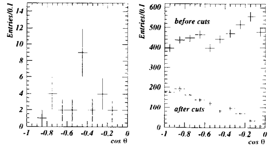
Fig. 20. \cos \theta distribution for events reconstructed as upward muons and passing the upward-muon cuts. Left side: experimental data. Right side: MC generated upward muons from interactions of atmospheric neutrinos. Full crosses: after reconstruction, but without any cuts; dashed crosses: after upward-muon cuts.
