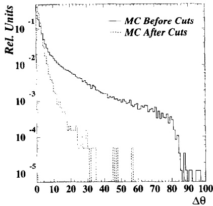
Fig. 16. Distribution of the zenith mismatch angle for NT-36 obtained from MC simulations of atmospheric muons.
