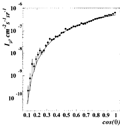
Fig. 17. Zenith angle distribution of the muon intensity I_\mu(\theta) at a depth of 1170 m. Full circles: experimental data, solid line: I_\mu(\theta) calculated for stochastic energy loss, respectively [43].
