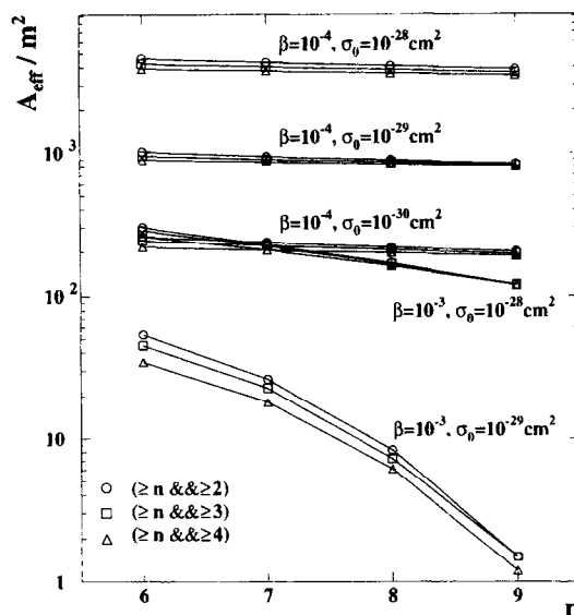
Fig. 23. Effective area for a single svjaska as a function of the trigger condition " N_{HIT}(1) \geq n AND N_{HIT}(2) \geq 2, 3, 4 " for different velocities \beta and catalysis cross sections \sigma_0 .
