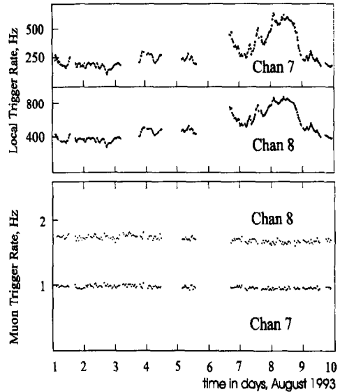
Fig. 9. a) Local trigger rates for channel 7 (downward facing) and channel 8 (upward facing) for August 1st-9th, 1993. The counting rates are averaged over 30 min. b) Muon trigger rates (condition 4/1) for channel 7 and 8. Counting rates are averaged over 50 min.
