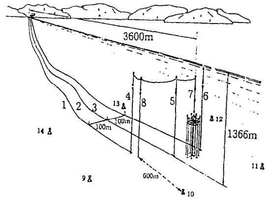
Fig. 3. The Baikal detector complex (status since 1994). 1,2 – wire cables to shore, 3 – opto-electrical cable to shore, 4,5,6 – string stations for shore cables 1,2,3, respectively, 7 – string with the telescope, 8 – hydrometric string, 9–14 – ultrasonic emitters.
