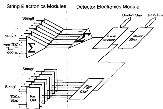
Fig. 7. Formation of the muon trigger.
