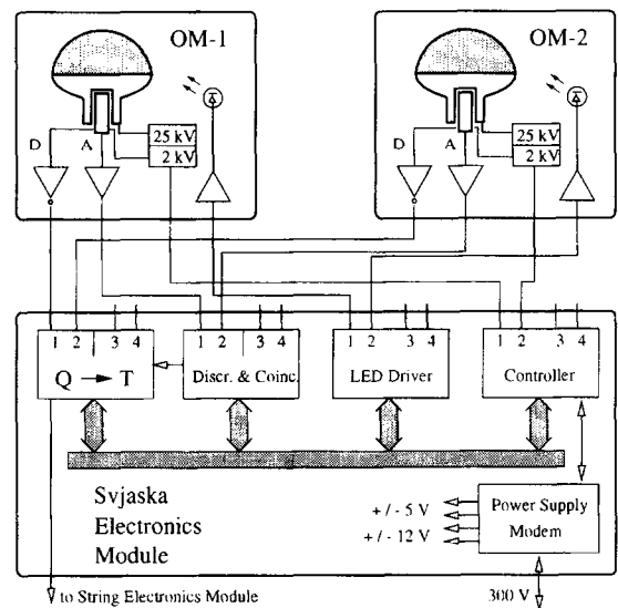
Fig. 6. Scheme of the svjaska electronics controlling 2 pairs of OMs (only the 2 PMTs belonging to the first pair are shown).
