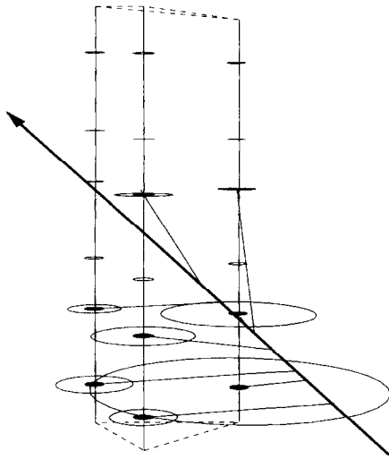
Fig. 19. An event recorded with NT-36 , reconstructed as upward muon and passing all cuts with the exception of the second upward-muon criterion. The time pattern of an upward muon (thick line) is likely to be faked by a shower just below the array yielding large amplitudes in the bottom channels.
