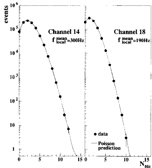
Fig. 21. Hit distributions in a time window of 8 ms, as recorded in a 2 h testrun for channels 14 and 18 of NT-36 . Experimental data are indicated by points, the curve gives the Poisson prediction.
