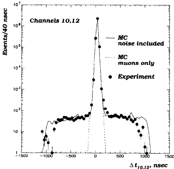
Fig. 12. Distribution of light arrival time differences \Delta t_{i,j} = t_j - t_i for channel 10 and 12 (string 2) for a muon run with trigger 4/1. Points are experimental data, lines are MC results without noise (dashed line) and with noise due to random hits (full line).
