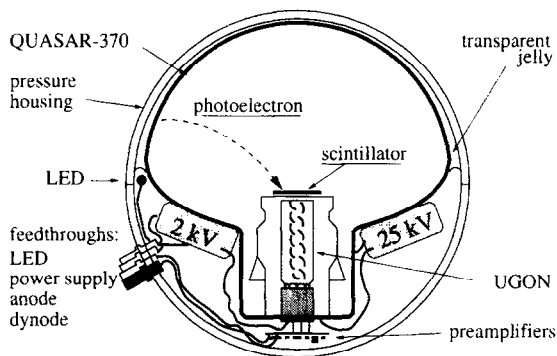
Fig. 5. The Optical Module of the Baikal experiment (see text for explanations).
