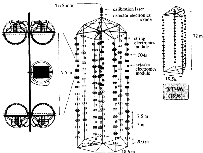
Fig. 4. Schematic view of the Baikal Telescope NT-200. The modules of NT-36, operating 1993/94 are in black, the modules added in 1995 are in grey. The expansion left-hand shows 2 pairs of optical modules ('svjaska') with the svjaska electronics module, which houses parts of the read-out and control electronics. Top right the array NT-96 is shown, which has been deployed in 1996.
