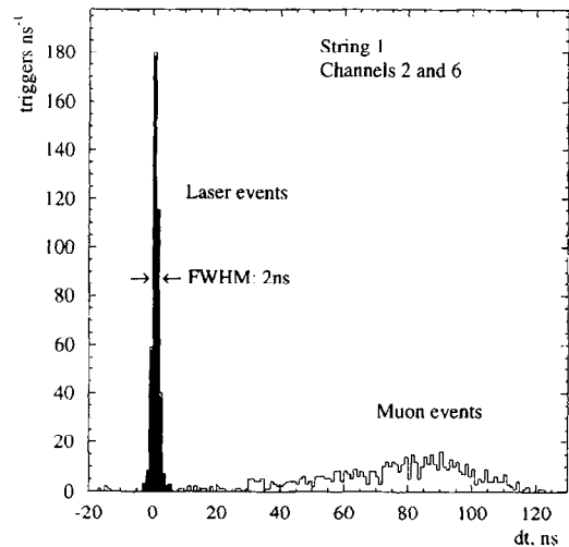
Fig. 11. Distribution of light arrival time differences \Delta t_{i,j} = t_j - t_i for channels 2 and 6 (string 1) for a typical laser run, with muon triggers recorded in parallel.
