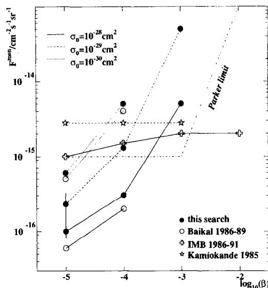
Fig. 24. Upper limits (90% CL) on the flux of magnetic GUT monopoles as a function of their velocity \beta , for different catalysis cross sections \sigma_0 .
