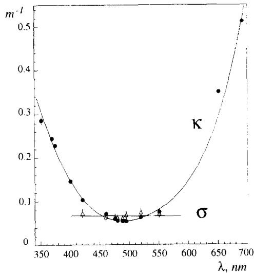
Fig. 2. Coefficients for light absorption ( \kappa ) (dots) and scattering ( \sigma ) (triangles) at the site of the Baikal Neutrino Telescope as a function of wavelength. Date of measurement: October/November 1993. Depth: 1100 m.
