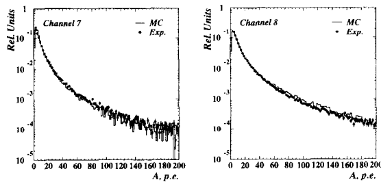
Fig. 14. Distribution of the amplitudes for channel 7 and 8. Points: experimental data, solid line: muons including full energy loss.
