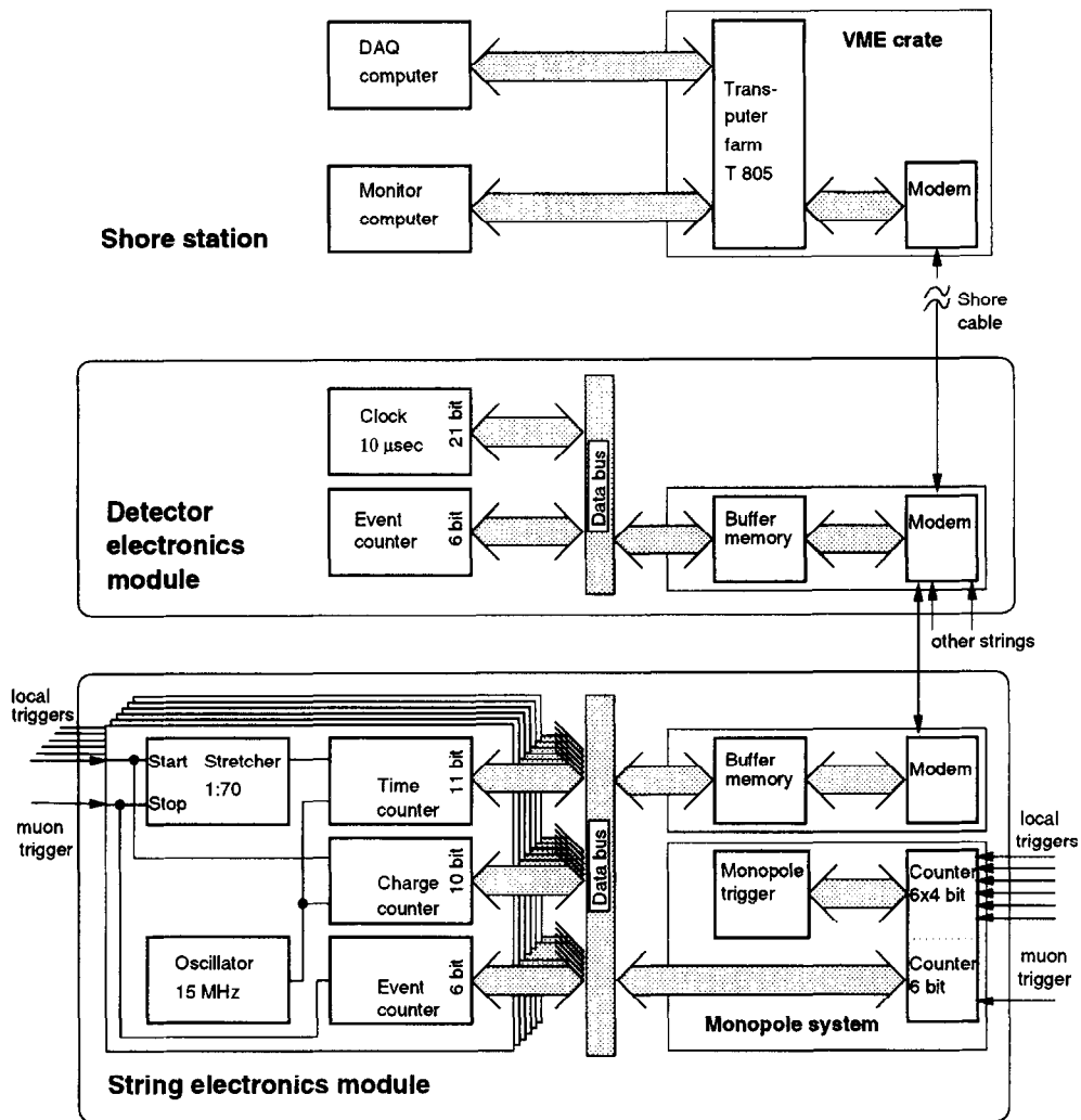
Fig. 8. Scheme of the NT-200 data acquisition system.
