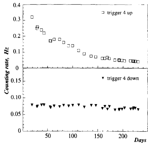
Fig. 10. Trigger rates over a period of 225 days starting with April 13th, 1993. Top: condition 4-up (at least 4 upward channels hit). Bottom: condition 4-down (at least 4 downward channels hit).
