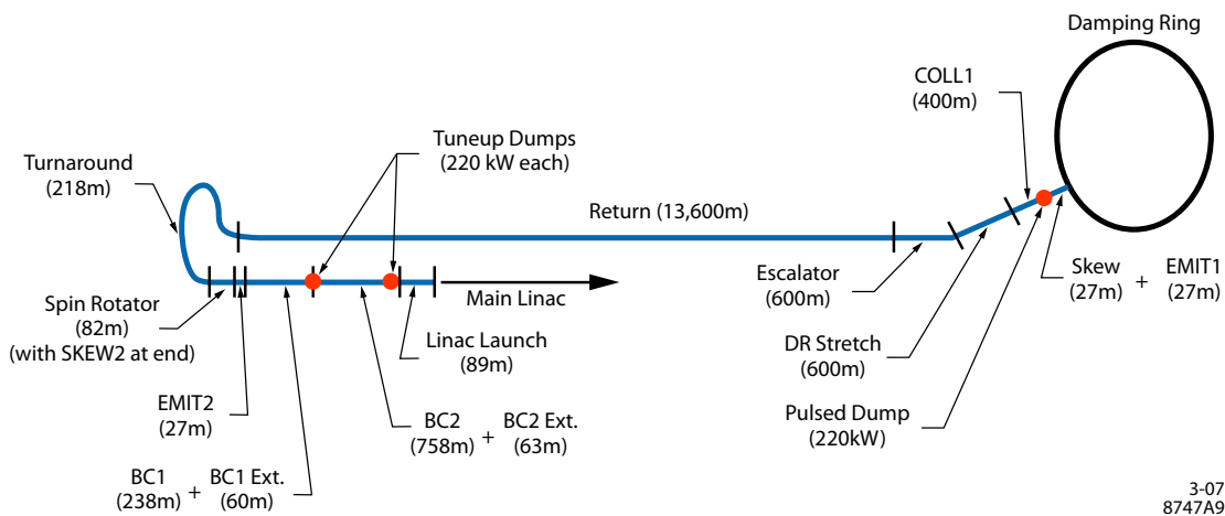
FIGURE 2.9. Schematic of the RTML.
