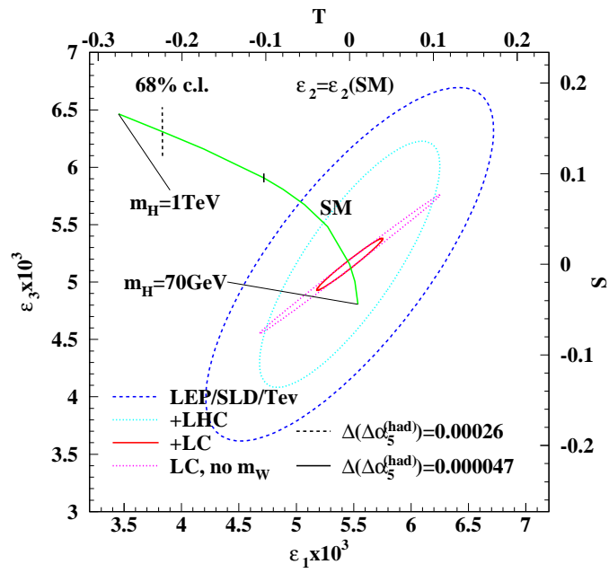
FIGURE 10.2. S-T ( \varepsilon_1 - \varepsilon_3 ) parameters now, after LHC and after GigaZ
