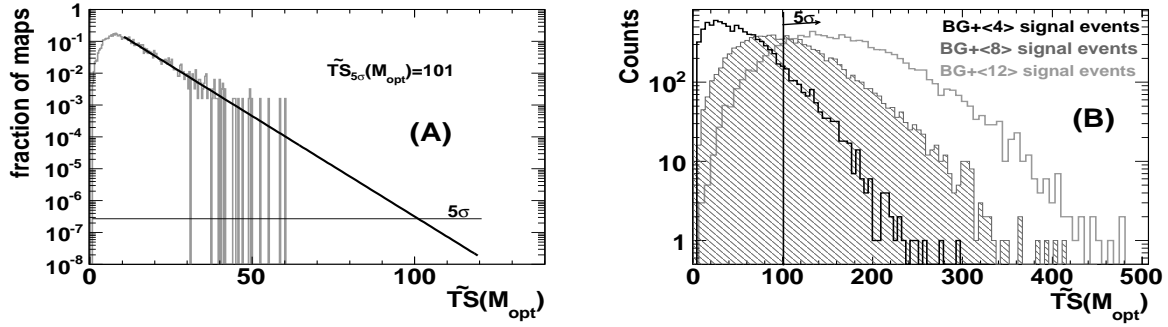
Figure 8: (A) Probability distribution of the global test statistics \widetilde{TS}(M_{opt}) for background-only simulations. The solid line shows an exponential fit to the distribution used to obtain the 5\sigma threshold for the background only case; (B) Distributions of the test statistic \widetilde{TS}(M_{opt}) for background plus signal simulations, where signal events are injected according to a Poisson distribution with mean: 4, 8, 12 signal events, respectively. The vertical line corresponds to the 5\sigma threshold.
