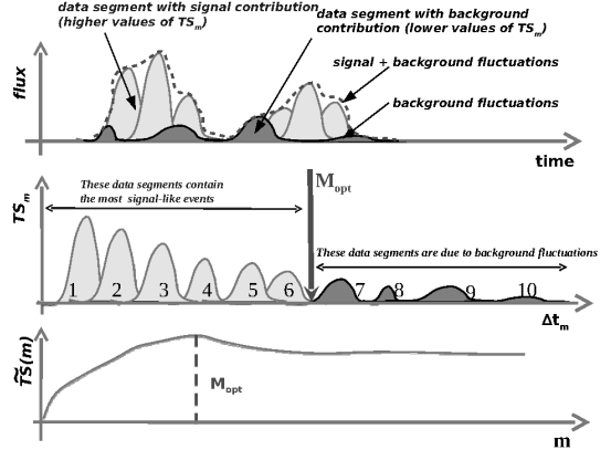
Figure 2: Sketch of the flare stacking procedure. Top: A data set is divided into segments being defined as in Figure 1. Some of these segment will include signal contribution, others background fluctuations only; Middle: Sorted values of the test statistic for each data segment from a maximization of the likelihood in Eq. (2) as a function of the data segment index m . Bottom: Evolution of the test statistic from a maximization of the likelihood in Eq. (8) as a function of the number of data segments being stacked following Eq. (9). The maximum value of this parameters defines the optimal number of data segments to be stacked M_{\text{opt}} .
