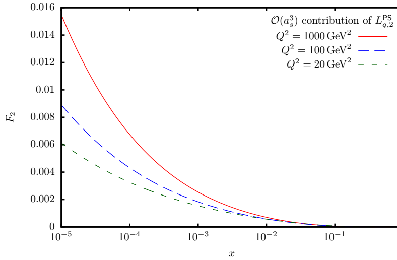
Figure 3: The O(a_s^3) contribution by L_{q,2}^{\text{PS}} to the structure function F_2(x, Q^2) .
