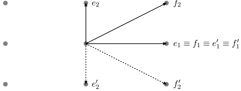
Figure 3: Two different bases for the p -rectangular lattice: \mathbf{e} = \{e_1, e_2\} and \mathbf{f} = \{f_1, f_2\} , and the action of the point group generator (primed vectors).
