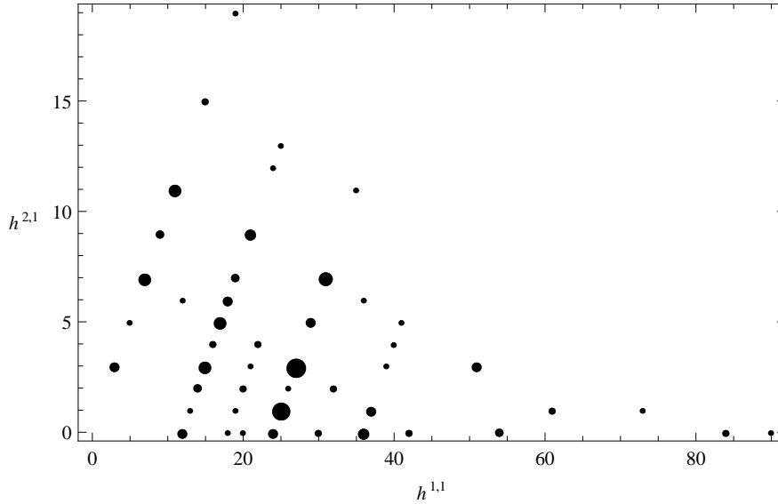
Figure 7: Statistics of the Hodge numbers for the 138 Abelian toroidal orbifolds of Table C.1.
