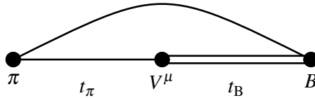
Figure 1: Quark line diagram for the three point function.
