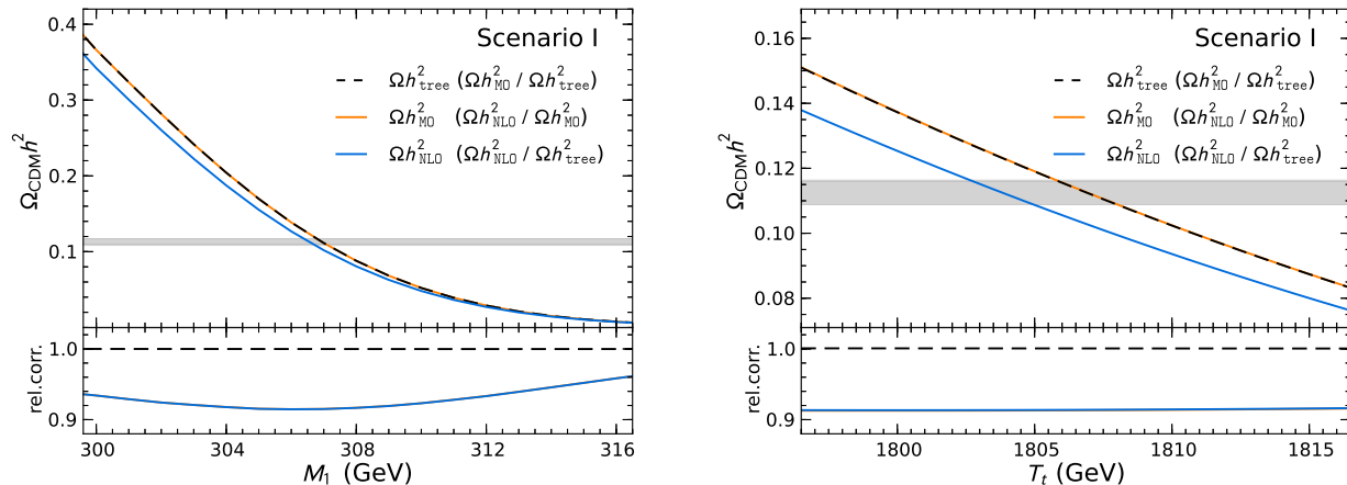
FIG. 11. The neutralino relic density \Omega_{\chi} h^2 as a function of M_1 (left) and T_t (right) in our scenario I calculated using different co-annihilation cross sections: default micrOMEGAs (orange solid line), tree-level (black dashed line), and full one-loop (blue solid line). The gray band indicates the favored range according to Eq. (1.1). The lower part shows the relative impact of the one-loop correction on the relic-density compared to the tree-level calculation.
