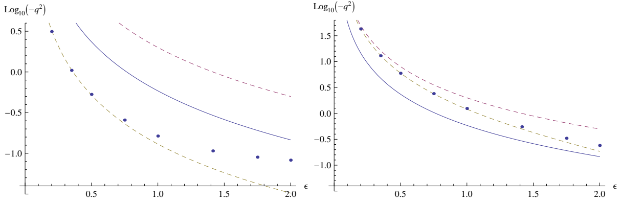
Figure 2: Tachyonic masses for unstable modes of n = 1 and n = 2 R-strings with \lambda = 1/2 . Dashed lines in the left panel are \epsilon^2 q^2 = -2, -2 \times 0.065 and dashed lines in the right panel are \epsilon^2 q^2 = -2, -2(1 - 0.39\epsilon^{2/3}) .
