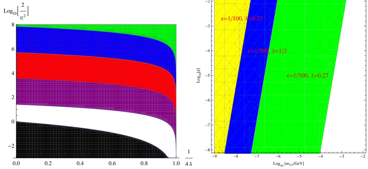
Figure 9: The regions corresponding to the case 1 in Figure 7, T_R^{\text{gr}} > T_B . We assume g_* = 220 . All winding strings are stable until the times of their decays. In the left panel the regions colored by purple, red, blue, and green correspond to (m_{3/2}/\text{GeV})\kappa^{-1/5} = 10^{-9}, 10^{-6}, 10^{-3}, 10^0 , respectively. A region with |m_X| > |m_\phi| is almost excluded by this strong condition.
