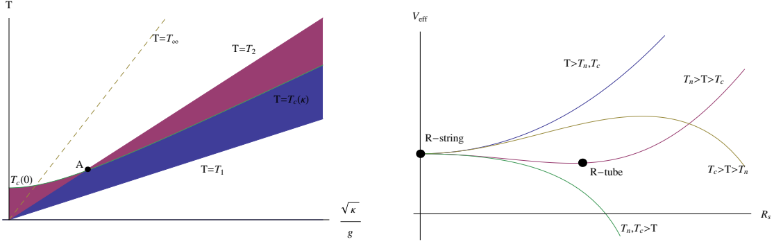
Figure 4: The left panel shows phases of R-string/R-tube. With a winding number n , an R-string is stable even including quantum effect at high temperature T > T_n, T_{cr} , and is unstable in any sense at T < T_{cr}, T_n . For T_{cr} > T > T_n , an R-string is classically stable and for T_n > T > T_{cr} an R-tube is stable.
