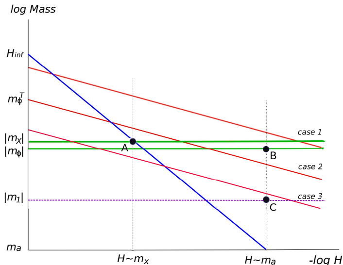
Figure 7: In the case 1, the reheating temperature is in T_R > T_B and the SUSY breaking vacuum is preferable. R-strings with all winding number are stable until their decay. In the case 2, the reheating temperature satisfies T_B > T_R > T_A > T_C . The vacuum selection is successful but some of higher winding R-strings are unstable. In the case 3, reheating temperature is lower T_A > T_R > T_C . The vacuum selection is unsuccessful when the tachyonic masses at the origin are |m_\phi| > |m_X| .
