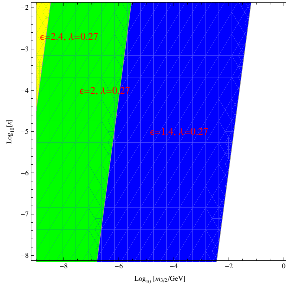
Figure 10: Three colored regions satisfy T_A > T_R^{\text{gr}} > T_C corresponding to the case 3 in Figure 7. We took \lambda = 0.27 and g_* = 220 . Tachyonic masses we used (q_1^2, \epsilon) = (10^{-5.4}, 1.4), (10^{-4.8}, 2), (10^{-4.3}, 2.4) .
