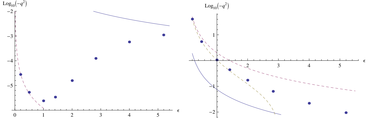
Figure 1: Tachyonic masses for unstable modes of n = 1 and n = 2 R-strings with \lambda = 0.27 . Solid lines represent \epsilon^2 q^2 = -2(1 - 1/\sqrt{4\lambda}) and a dashed line in the left panel is \epsilon^2 q^2 = -2 \times 6 \times 10^{-7} and dashed lines in the right panel are \epsilon^2 q^2 = -2, -2(1 - 0.47\epsilon^{2/3}) .
