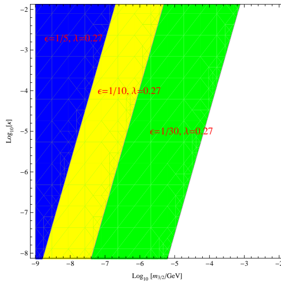
Figure 8: The regions satisfying the condition T_B > T_R^{\text{gr}} > T_A (> T_C) that correspond to to the case 2 in the Figure 7. We take g_* = 220 by assuming the messengers are not thermalized.
