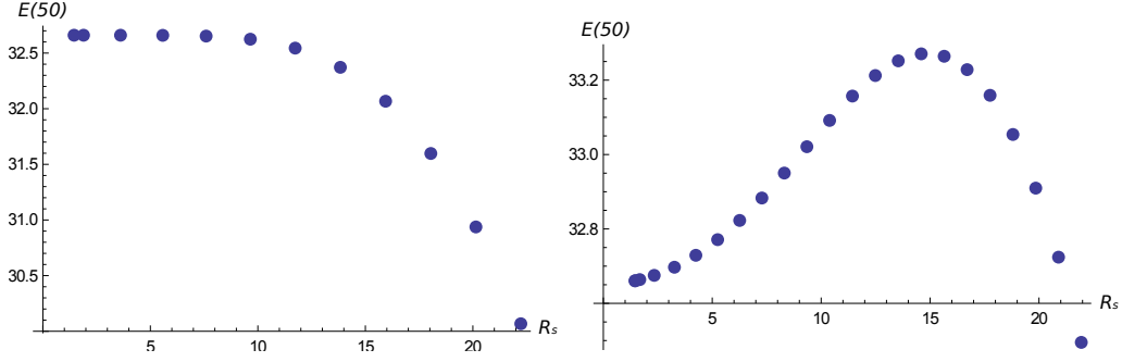
Figure 3: The low energy effective theory for \lambda = 0.27 , \epsilon = 1 and n = 1 . Left panel is for almost zero temperature k = 0.001 . Right panel is for k = 0.01 .
