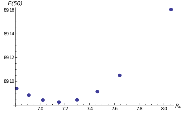
Figure 5: R -tube solution with n = 2 , k = 0.5 , \lambda = 0.27 , \epsilon = 1 . A minimum exists around R_s \sim 7.2 .
