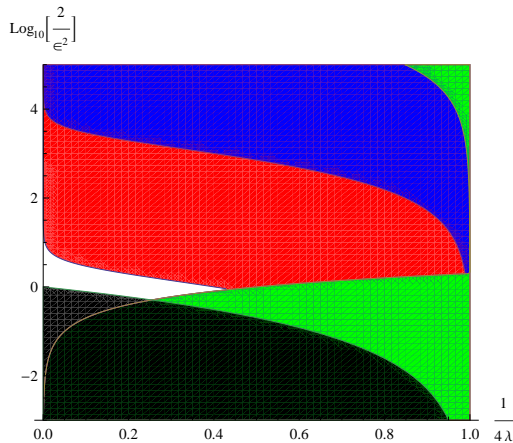
Figure 6: The region satisfying one of the two inequality T_R^{\text{gr}} > T_A (defined in (4.12)) and |m_X| > |m_\phi| with (m_{3/2}/\text{GeV})\kappa^{-1/3} = 10^{-6}, 10^{-3}, 10^0 which are colored by red, blue, and green respectively. The black region is excluded by the condition of the existence of the SUSY breaking vacuum.
