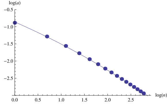
Figure 11: Dots are numerical data of a = \tilde{a}_n and a solid line gives a = 1/\sqrt{4.5n + 1.1n^2} .
