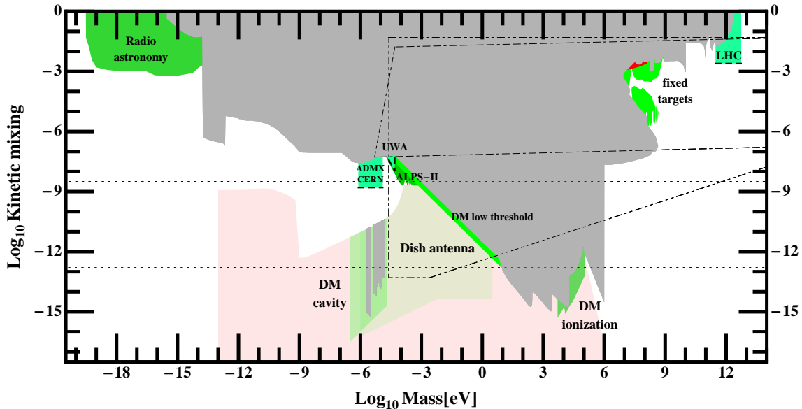
Fig. 3: Parameter space for hidden photons (HPs). The grey region indicates the parameter space already excluded by different experiments, see [3] for details. The reddish area in the bottom indicated the region in which HPs could constitute Cold Dark Matter. Various shades of green correspond to parameter regions accessible by planned and proposed experiments.
