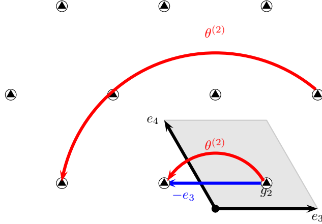
Figure 3: Visualization of the geometrical eigenstate |[g_2]\rangle of equation (23). One performs a sum over all equivalent fixed points in covering space weighted by appropriate \gamma phase factors. The sublattice rotation \theta^{(2)} is, for g_2 , geometrically equivalent to a lattice translation by -e_3 up to three times a lattice translation.
