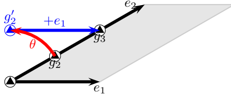
Figure 2: The second twisted sector in the G_2 two-torus has three fixed points (black dots) with corresponding constructing elements g_a , a = 1, 2, 3 . Under \theta the fixed point of g_2 is mapped to g'_2 , which is equivalent to g_3 by a lattice translation +e_1 . Hence, the constructing elements g_2 and g_3 belong to the same conjugacy class.
