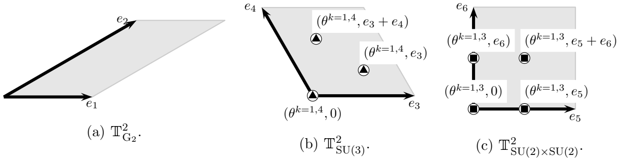
Figure 1: The factorized lattice \Lambda of the six-torus is chosen to be spanned by the roots of G_2 \times SU(3) \times SU(2)^2 . The six vectors e_\alpha denote a basis. For later convenience, we show also the fixed points in the SU(3) and SU(2) \times SU(2) planes.
