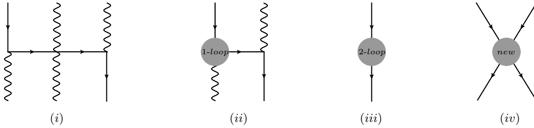
Figure 5: At two-loops, the types of diagrams that contribute to the renormalization of operators are bare skeleton diagrams of order g^4 , one-loop self-energy and vertex corrections to the tree-level skeleton diagrams of order g^2 that appeared in the one-loop order (dressed skeletons) and two-loop self-energy corrections. What is more, operators can be renormalized by new vertices that appear for the first time in the effective action at one-loop.
