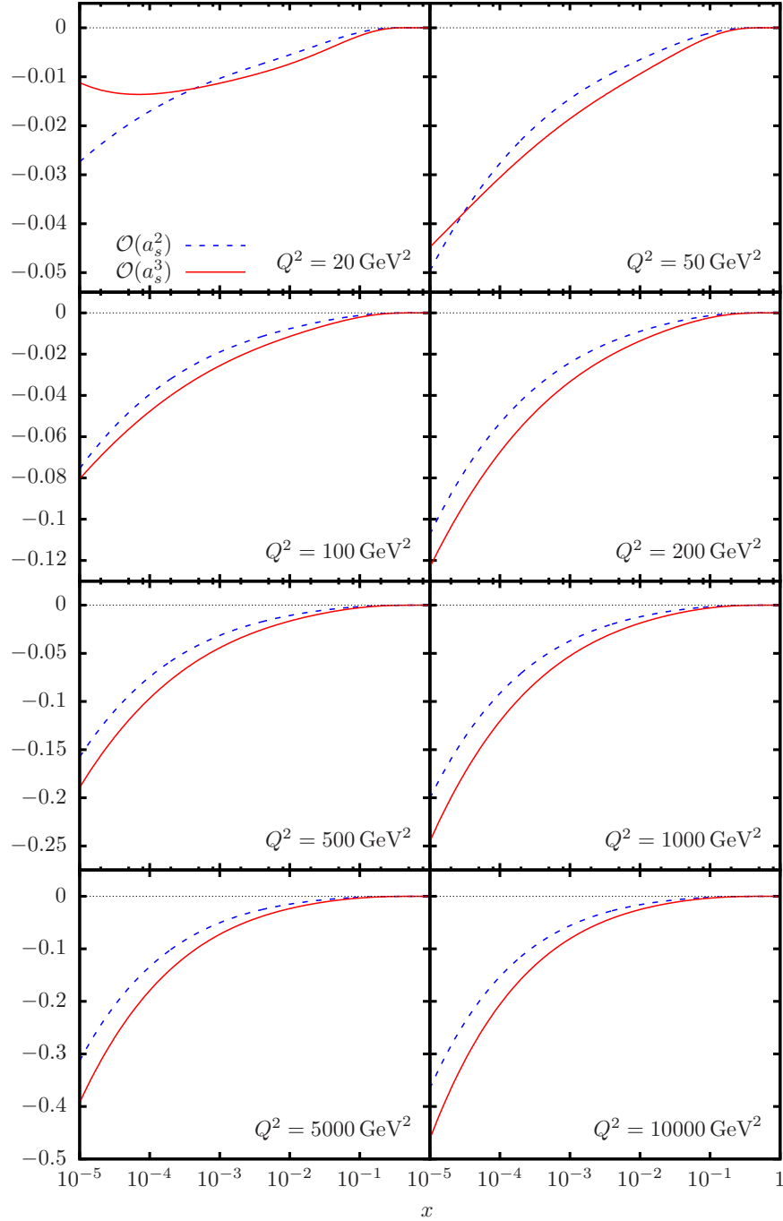
Figure 10: The charm contribution by the Wilson coefficient H_{Q,2}^{\text{PS}} to the structure function F_2(x, Q^2) as a function of x and Q^2 choosing Q^2 = \mu^2 , m_c = 1.59 \text{GeV} (on-shell scheme) using the parton distribution functions [4].
