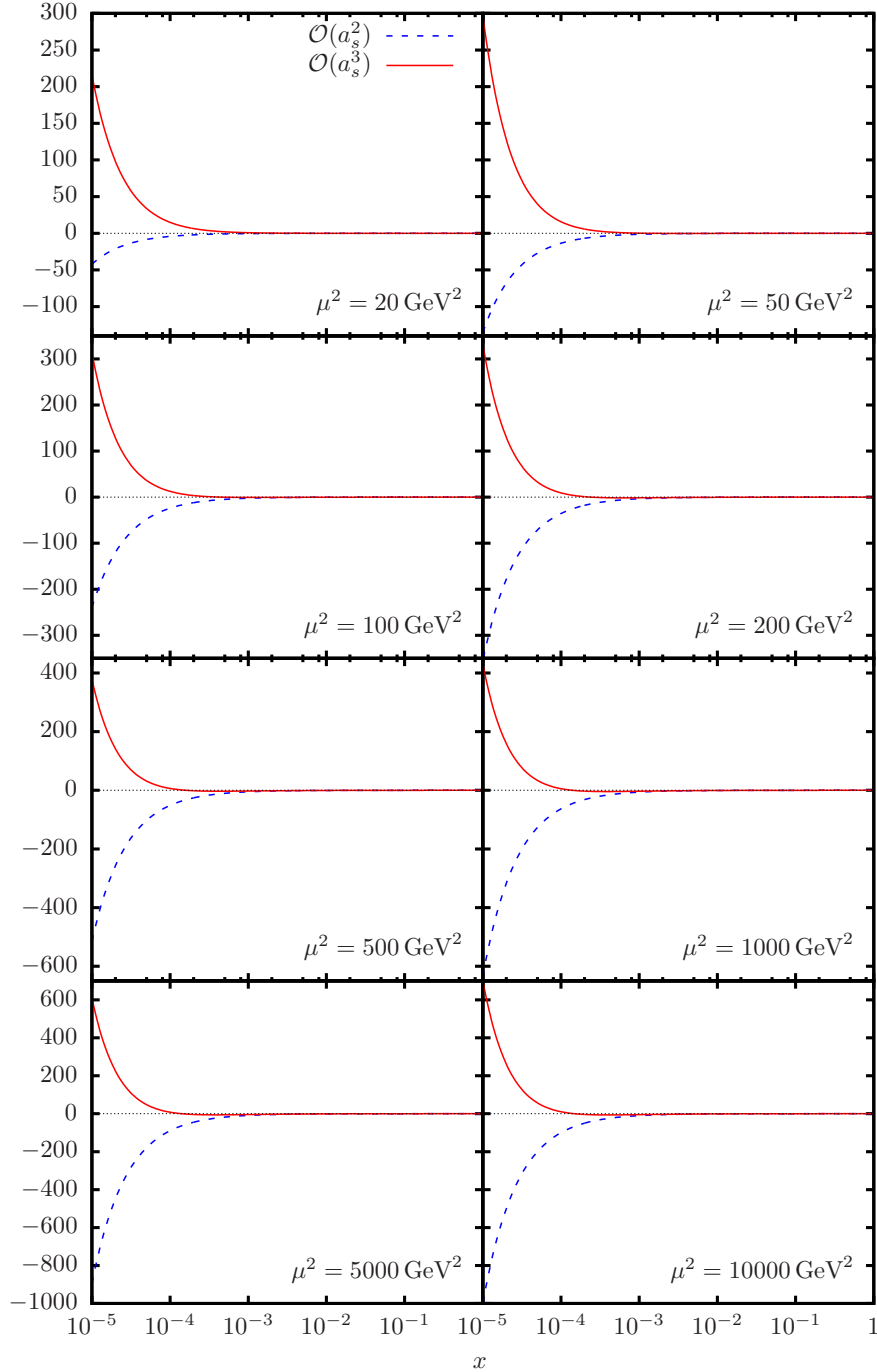
Figure 6: The OME A_{Qq}^{\text{PS}} up to 2- and 3-loop order in dependence of x and \mu^2 for a heavy quark mass m_c = 1.59 GeV (on-shell scheme), cf. [5].
