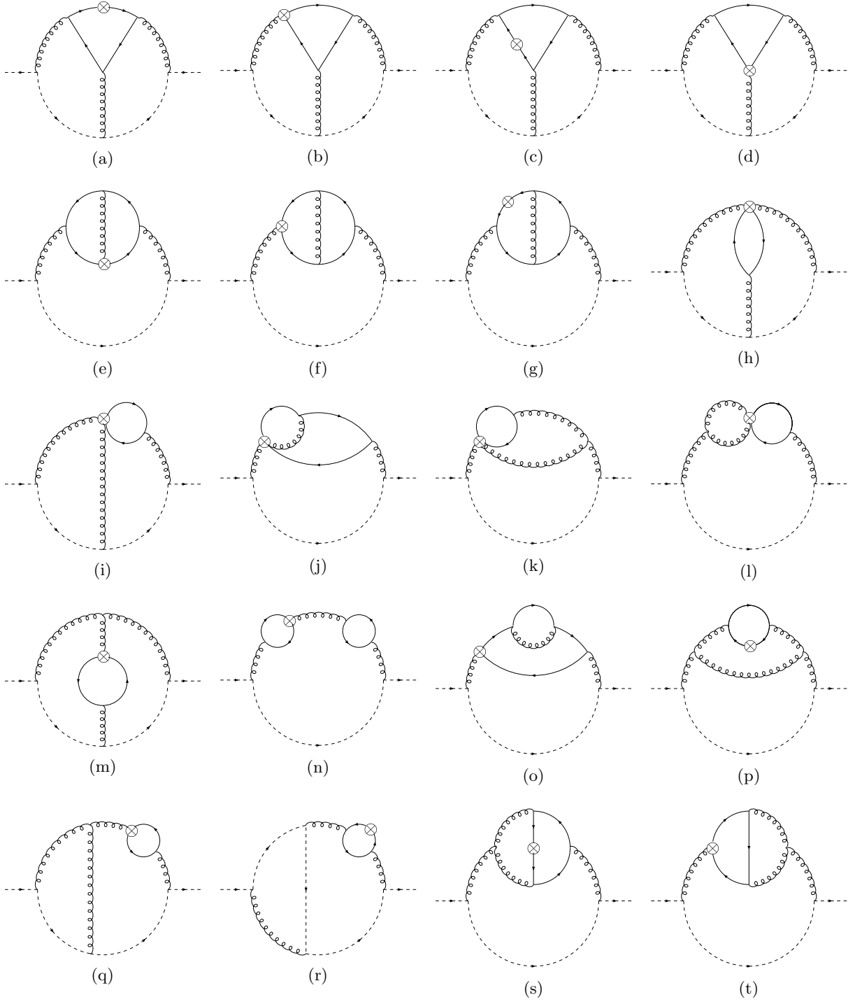
Figure 1: Sample of diagrams for A_{Qq}^{(3),\text{PS}} . The dashed arrow lines represent massless quarks, while the solid arrow lines represent massive quarks, and curly lines are gluons. In terms of Feynman integrals, diagrams (a–j) represent the main topologies, in other words, other diagrams, such as diagrams (k)–(t) can be seen as sub-topologies and/or are related to diagrams (a–j) by symmetry. The symbol \otimes denotes the local operator insertion, see Ref. [12].
