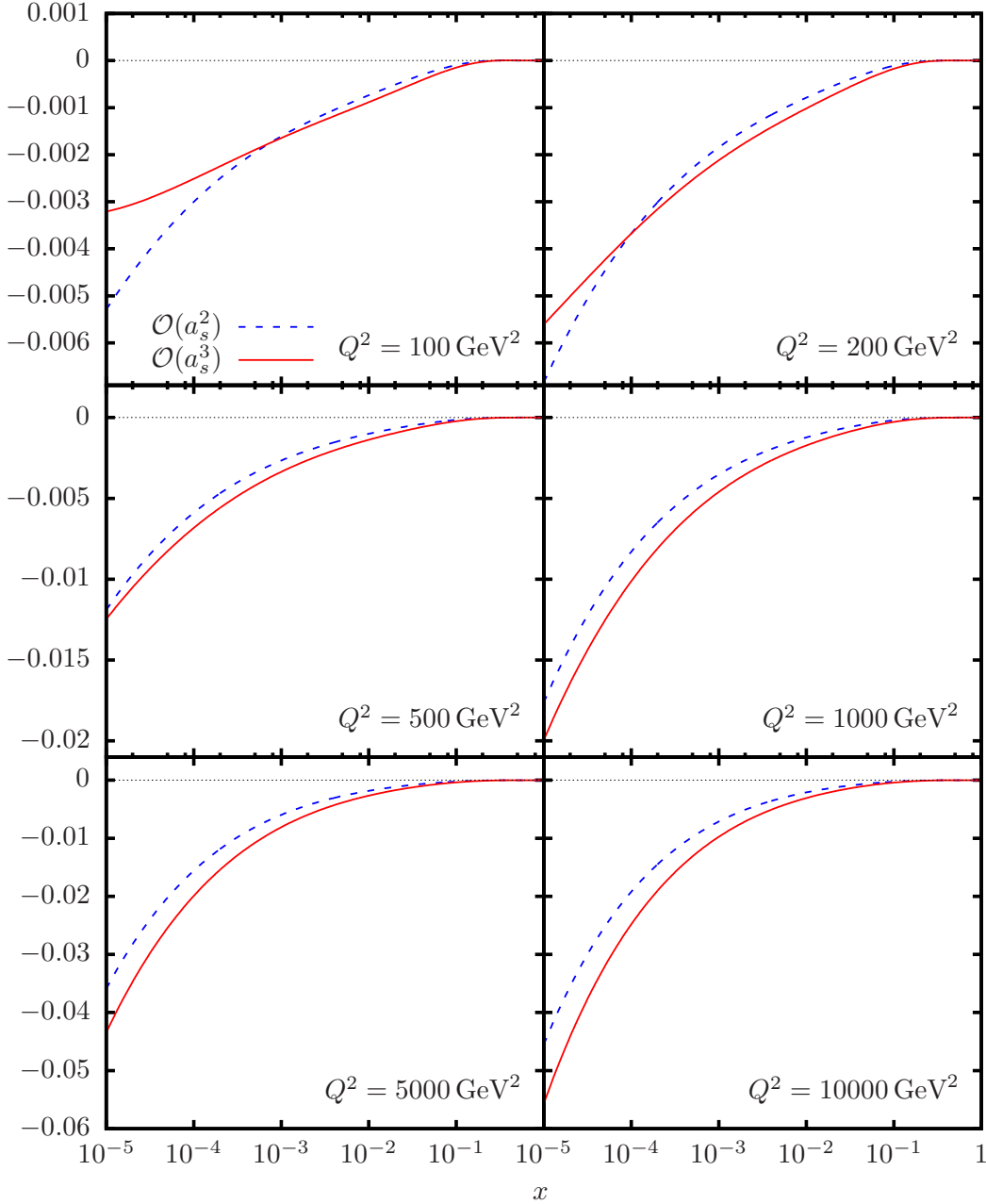
Figure 11: The bottom contribution by the Wilson coefficient H_{Q,2}^{\text{PS}} to the structure function F_2(x, Q^2) as a function of x and Q^2 choosing Q^2 = \mu^2 , m_b = 4.78\text{GeV} (on shell scheme [112]) using the parton distribution functions [4].
