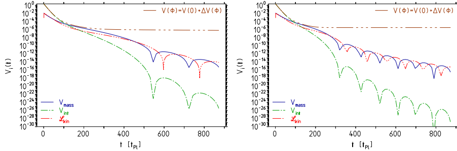
Figure 6: The mass-, interaction- and kinetic-term of the bare Lagrangian in units of M_{\text{Pl}}^4 as a function of time. Left: the relative contributions when proper running of SM couplings are taken into account. The mass term is dominating in the range t \simeq 100 to 450 t_{\text{Pl}} , where the slow-roll era ends and damped quasi-free field oscillations start. Right: fake solution based on constant couplings.
