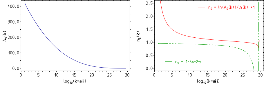
Figure 9: The spectral amplitude A_S(k) as a function of k = aH [left] and a comparison of the indices n_S = \ln A_S(k)/\ln k + 1 versus n_S = 1 - 6\varepsilon + 2\eta [right].
