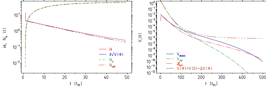
Figure 2: The inflation era. Left: N_e \approx 66 is reached at time t \approx 50 t_{\text{Pl}} . The Hubble constant H is satisfying H \approx \ell \sqrt{V(\phi)} very well shortly after Planck time. The evaluation of N_e via Eq. (21) agrees very well with the numerical N_{\text{eff}} = \ln a(t)/a(t_{\text{Pl}}) obtained by solving the coupled set of dynamical equations. Right: dark energy contributions during inflation. Shown are the separate terms of the Higgs potential together with the Higgs kinetic term. Slow-roll inflation stops at about t \approx 450 t_{\text{Pl}} when \mathcal{L}_{\text{kin}} \sim V_{\text{mass}} \gg V_{\text{int}} , after which the Higgs behaves as a damped quasi-free oscillating field.
