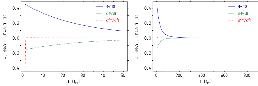
Figure 5: The Higgs field and its derivatives for k = 1 as a function of time all in units of the Planck mass. Left: the Higgs field at start. Right: the Higgs field decay before the Higgs transition. The field starts oscillating strongly like a free field once \mathcal{L}_{\text{kin}} \sim V_{\text{mass}} while V_{\text{int}} \ll V_{\text{mass}} (see Fig. 6).
