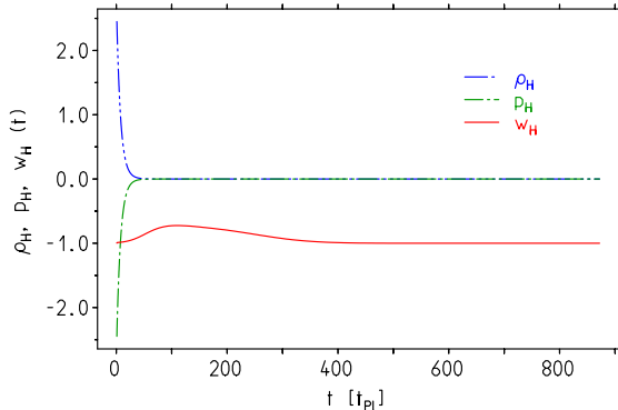
Figure 7: Higgs field density, pressure and equation of state. The Higgs provides dark energy beyond the inflation period which ends at about t \simeq 450 t_{P1} .
