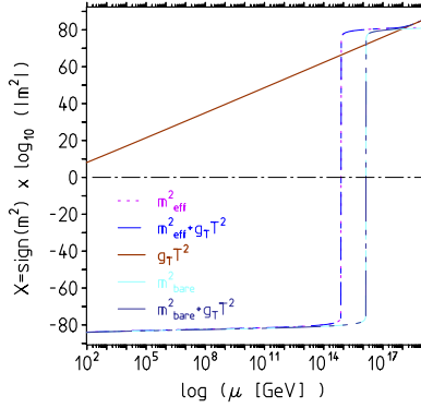
Figure 13: The effective mass vs. the bare mass including finite temperature effects. The latter have little effect on the location of the EW phase transition. The shift C_1 \rightarrow C'_1 = C_1 + \lambda has a substantial effect on the scale of the Higgs transition.
