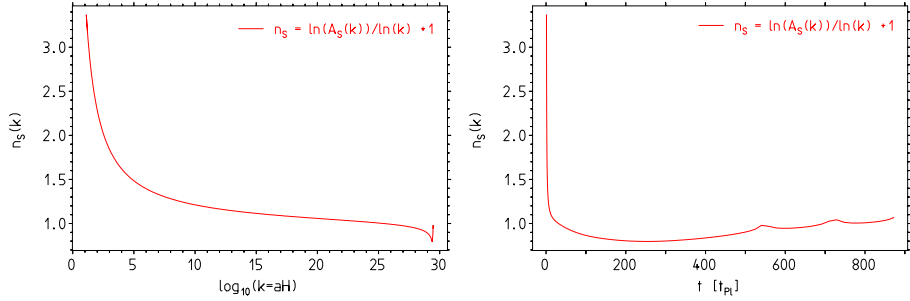
Figure 10: The index n_S(k) extracted from A_S(k) as a function of k = aH [left] and as a function of time t in units of t_{P1} .
