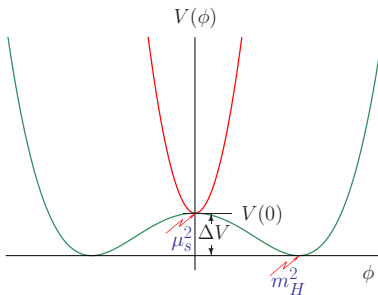
Figure 11: Vacuum rearrangement of the Higgs potential. At the zero of X(\mu) of Eq. (63) \Delta V = -V(0) nullifying the difference between bare and renormalized CC. The bare mass m^2 = \mu_s^2 in the symmetric phase is not correlated to renormalized m_H^2 in the Higgs phase, as also the difference between the two masses vanishes at the Higgs transition point.
