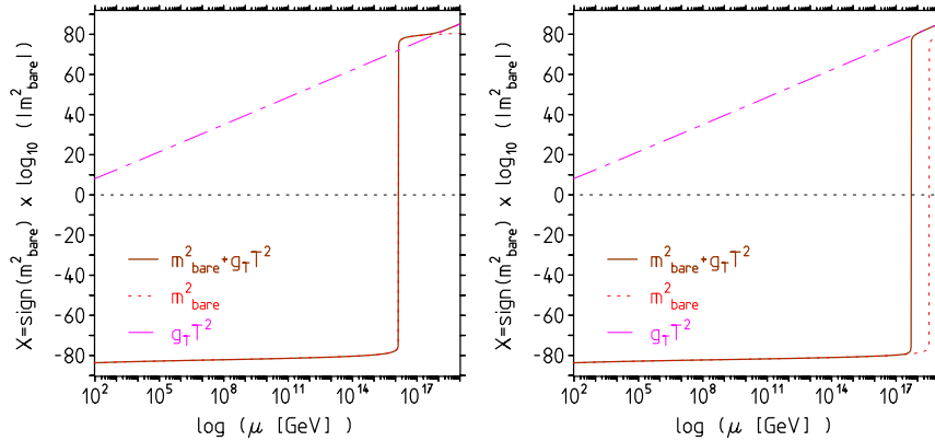
Figure 1: The role of the effective bare mass in the finite temperature SM. Left: for \mu_0 \sim 1.4 \times 10^{16} GeV ( M_H \sim 126 GeV, M_t \sim 173.5 GeV). Right: finite temperature delayed transition for \mu_0 \sim 6 \times 10^{17} GeV ( M_H \sim 124 GeV, M_t \sim 175 GeV), the m_{\text{bare}}^2 term alone is flipping at about \mu_0 \sim 3.5 \times 10^{18} GeV. Inflation requires m_b^2 > g_T T^2 !
