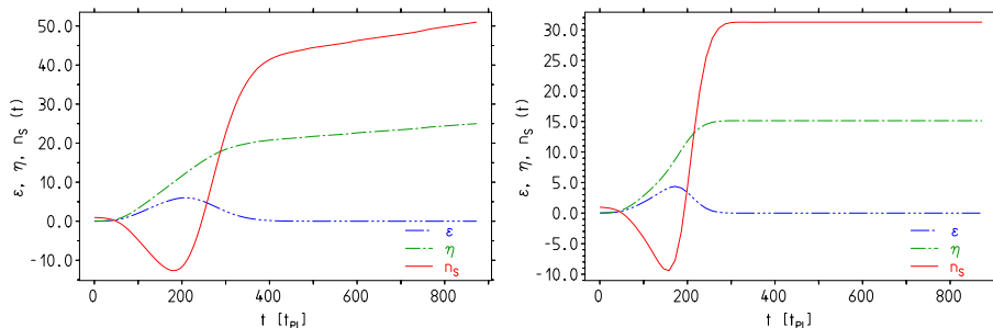
Figure 8: The slow-roll coefficients \epsilon , \eta and the spectral index n_S = 1 - 6\epsilon + 2\eta for the scalar fluctuations, as a function of time before the bare Higgs transition point. Left: correct result taking into account the running couplings. Right: fake results assuming fixed couplings as given at the Planck scale.
