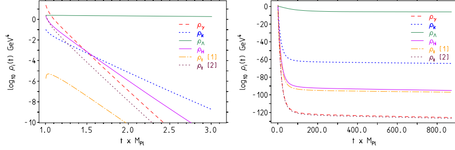
Figure 3: Right: this graph shows that the dark energy term as given by (1) is dominating the density quite soon after the big bang, and thus indeed is driving inflation. Left: analogous plot taking into account the Higgs decay into t\bar{t} [1] up to before the Higgs transition ( \phi_0 \simeq 4.5 M_{\text{Pl}} ). \rho_t [2] (in the plot little below \rho_\gamma ) is the top component in \rho_\gamma , which denote the total radiation density without the reheating part. For later reference we also show the top quark density \rho_t obtained from reheating [1] in comparison with the fraction of top quark radiation which is part of \rho_\gamma . Included is also the non-relativistic heavy Higgs component \rho_H given by Eq. (51).
