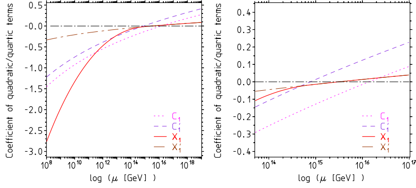
Figure 12: The correlated zeros of C_1(\mu) in the quadratic and of X_1(\mu) in the quartic Planck cutoff enhanced terms, respectively. Relevant are the effective coefficients C'_1 = C_1 + \lambda and X_1 . Here X'_1 represents the quartic coefficient not including the vacuum rearrangement jump, which does not actually affect the location of the zero.
