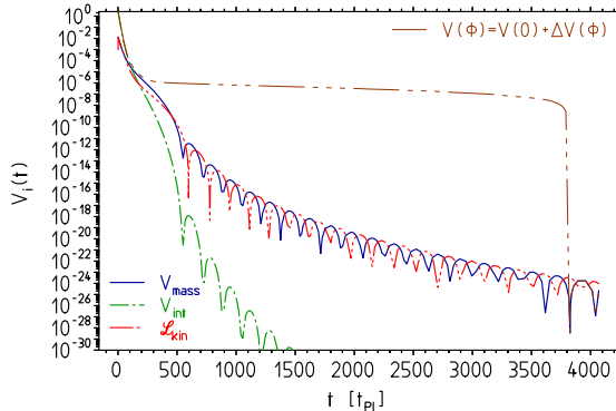
Figure 14: Here we show the same quantities as in Fig. 6 in an extended range exhibiting the vacuum rearrangement at \mu_{CC} . After inflation the scene is characterized by a free damped harmonic oscillator behavior. Relevant scales are \mu_0 \simeq 1.4 \times 10^{16} \Leftrightarrow t \simeq 870 M_{\text{Pl}}^{-1} at the zero of m_{\text{bare}}^2 - m_{\text{ren}}^2 = 0 , \mu_{CC} \simeq 3.1 \times 10^{15} \Leftrightarrow t \simeq 4000 M_{\text{Pl}}^{-1} where \rho_{\Lambda \text{ bare}} = \rho_{\Lambda \text{ ren}} and \mu'_0 \simeq 7.7 \times 10^{14} \Leftrightarrow t \simeq 15844 M_{\text{Pl}}^{-1} the true Higgs transition point m'^2 = 0 .
