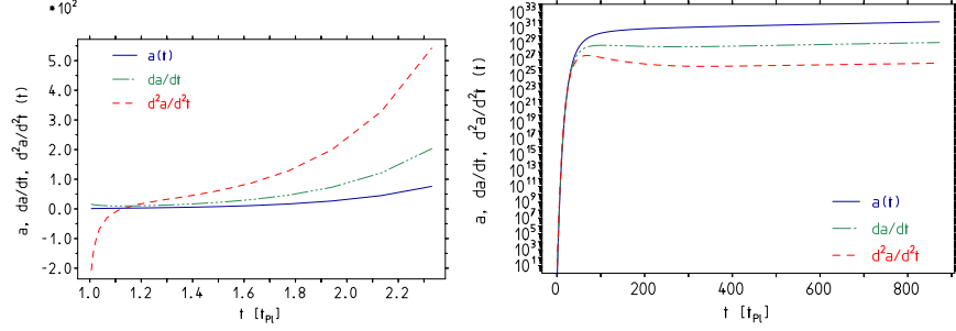
Figure 4: The FRW radius and its derivatives for k = 1 as a function of time all in units of the Planck mass, i.e. for M_{\text{Pl}} = 1 . Left: the start. Right: the expansion before the Higgs transition.
