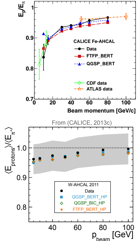
FIG. 73 Ratio of AHCAL response to protons relative to pions, as a function of beam momentum, for steel (top) and tungsten (bottom) absorber. From (Bilki et al. , 2015a) (top), (CALICE, 2013c; Sicking, 2013) (bottom).
