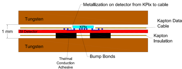
FIG. 7 The layer structure of the SiD Silicon-Tungsten Electromagnetic Calorimeter.
