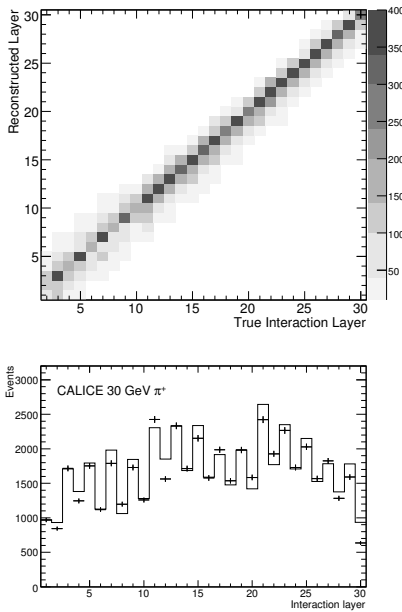
FIG. 62 Top: Comparison between the interaction layer reconstructed in the SiW ECAL and the interaction layer as extracted from the GEANT4 event record. This example corresponds to a 20 GeV \pi^- beam simulation, using the QGSP_BERT physics list. Bottom: Distribution of the reconstructed interaction layer in the ECAL for 30 GeV data (points), compared with Monte Carlo predictions using the QGSP_BERT physics list (solid histogram). From (Adloff et al. , 2010b).
