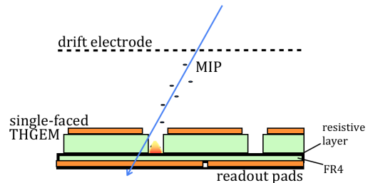
FIG. 13 A thick-GEM structure which provides discharge protection.
