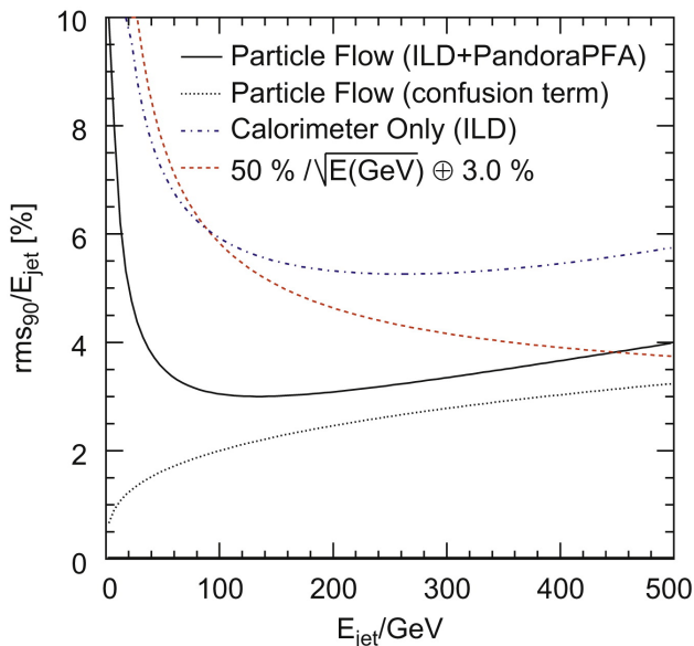
FIG. 4 Empirical form of the simulated ILD jet energy resolution as a function of energy. Also shown is the contribution from confusion, and, for comparison, the resolution obtained from the ILD calorimeter alone, and that of an ideal calorimeter with given parameters. From (Thomson, 2009).
