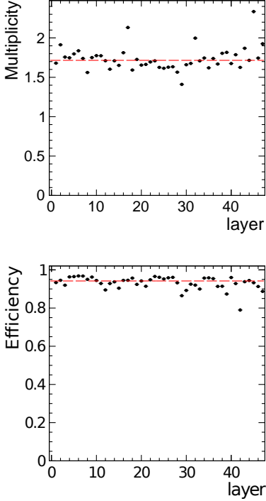
FIG. 42 Top: Average hit multiplicity in the CALICE SDHCAL chambers as a function of the layer. Bottom: Average efficiency of the CALICE SDHCAL chambers as a function of the layer. From (Boudry, 2012; CALICE, 2012b).
