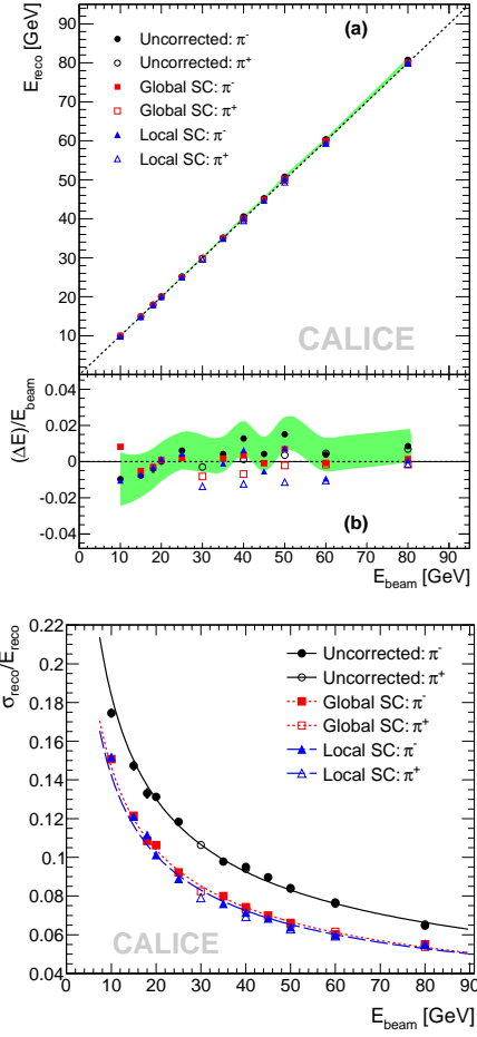
FIG. 49 Linearity and resolution for unweighted AHCAL data, and for the two software compensation methods. From (Adloff et al. , 2012c).
