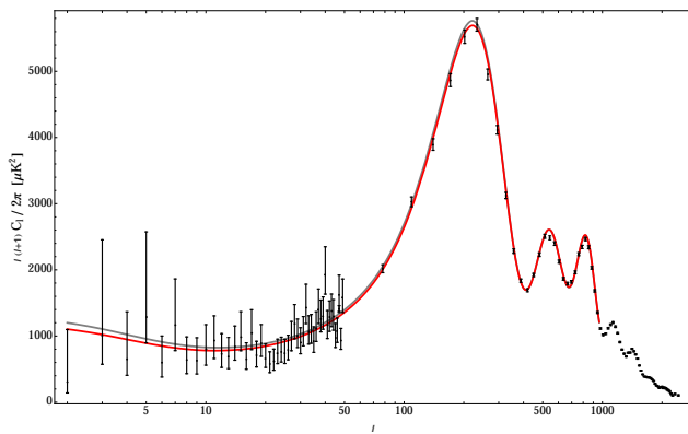
FIG. 5. Comparison of a model (11) with additional steepening from the \xi -dependent correction in the Kähler potential (12) with the Planck 2013 CMB temperature data. The grey line shows a reference prediction from a \Lambda CDM pure power-law power spectrum with n_s = 0.96 . The red line gives the prediction of our model with a = 0.105 , b = 0.263 and \xi = -0.0055 . This model provides n_s \simeq 0.98 and r \simeq 0.1 at N_e = 50 e-folds before the end of inflation, and generates a power suppression at low- \ell of about 10%. We see that the power suppression is confined to a relatively small range of low \ell 's , because the small \xi -correction generates an exponentially steep term in the scalar potential at large \phi .
