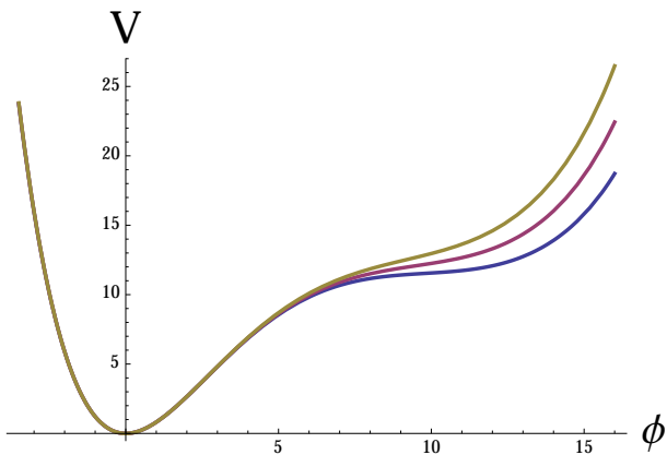
FIG. 2. The potential V(\phi) = \frac{m^2\phi^2}{2} (1 - a\phi + a^2b\phi^2)^2 for a = 0.1 and b = 0.36 (upper curve), 0.35 (middle) and 0.34 (lower curve). The potential is shown in units of m , with \phi in Planckian units. For each of these potentials, there is a range of values of the parameter a such that the observational predictions of the model are in the region of n_s and r preferred by Planck 2013. For b = 0.34 , the value of the field \phi at the moment corresponding to 60 e-foldings from the end of inflation is \phi \approx 8.2 . Change of the parameter a stretches the potentials horizontally without changing their shape.
