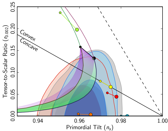
FIG. 1. The green area describes observational consequences of inflation in the Higgs model (10) with v \gg 1 ( a \ll 1 ), for the inflationary regime when the field rolls down from the maximum of the potential. The continuation of this area upwards corresponds to the prediction of inflation which begins when the field \phi initially is at the slope of the potential at |v - \phi| \gg v . In the limit v \rightarrow \infty , which corresponds to a \rightarrow 0 , the predictions coincide with the predictions of the simplest chaotic inflation model with a quadratic potential \frac{m^2}{2}\phi^2 .
