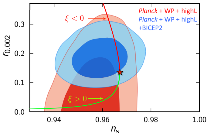
FIG. 6. Predictions for n_s and r for the theory \frac{m^2}{2}\phi^2 nonminimally coupled to gravity.
