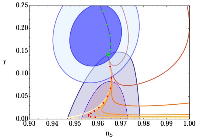
FIG. 3. Predictions for n_s(a) and r(a) in at 55 e-folds the model with V(\phi) = \frac{m^2\phi^2}{2} (1 - a\phi + a^2b\phi^2)^2 for various values of b = 0.334 \dots 5 . All curves have a running from 0.001 to 0.2. The red ( b = 0.34 ) and green ( b = 5 ) balls correspond to a = 0.01 \dots 0.13 in steps of 0.01 from the joint start point a = 0.001 outward. For a = 0 one recovers the predictions for the simplest chaotic inflation model with a quadratic potential for all b , while for b = 0.34 and a = 0.13 the predictions almost exactly coincide with the predictions of the Starobinsky model and the Higgs inflation model (red balls). Conversely for b \gtrsim 1 and moderately small a our model nicely traverses the BICEP2 constraints within the 1- \sigma area (green balls).
