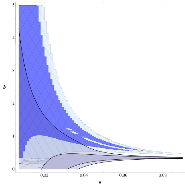
FIG. 4. Grey: Exclusion contours for the microscopic parameters (a, b) in the model with V(\phi) = \frac{m^2\phi^2}{2}(1 - a\phi + a^2b\phi^2) 2 from the PLANCK+WP+BAO approximated exclusion limits on n_s, r . Dark grey and light grey denote the 68% and 95% confidence level exclusion contour plot for the microscopic parameters (a, b) , respectively, conditioned on m chosen to keep COBE normalization of the curvature perturbation power.
