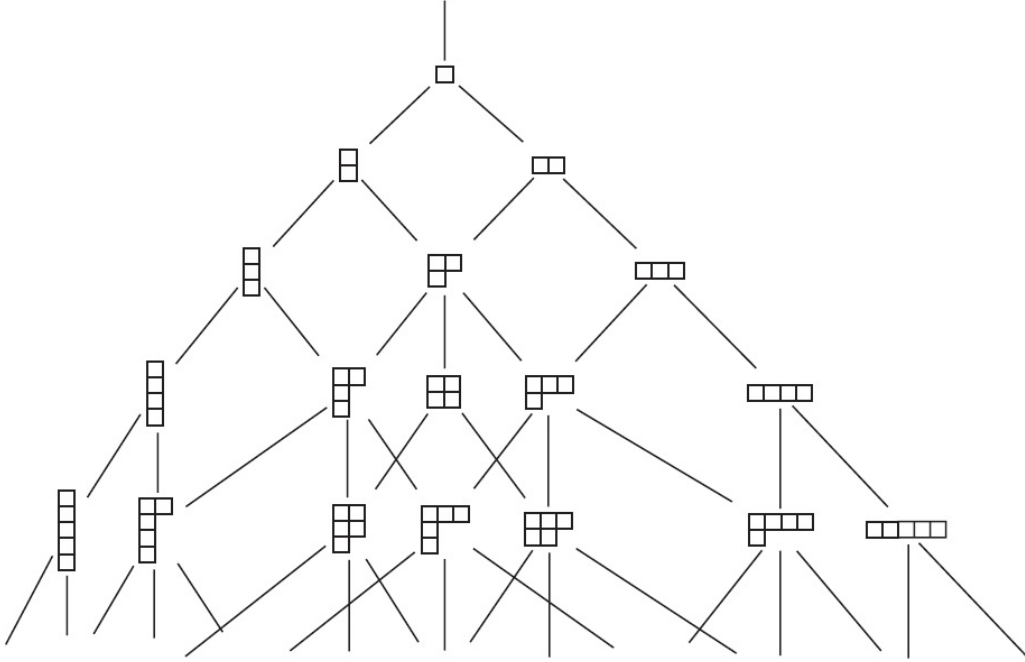
Figure 5: Hasse diagram of the Young lattice.
