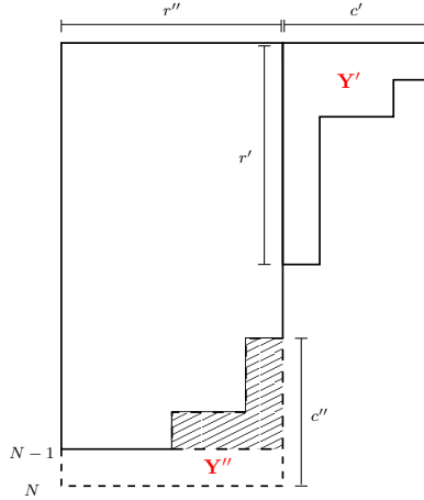
Figure 3: The Young diagram Y is obtained from a rectangle of size N \times r'' by attaching the Young diagram Y' and removing (a reflected version of) the Young diagram Y'' . Note that r' + c'' \leq N is needed for the resulting diagram to be a Young diagram of SU(N) . The shaded region shows those boxes from the tensor power of the dual fundamental that must be moved to the left.
