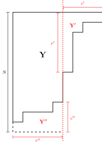
Figure 1: Dissecting the Young diagram Y by the red dashed line identifies Young diagrams Y' and Y'' as soon as their numbers of boxes match. This can happen exactly once.
