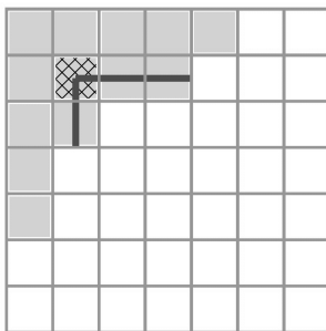
Figure 4: For each box (l, m) in the Young diagram Y , one can draw a hook. In the figure we have shaded the box and indicated the hook by the thick line. The length of the hook, i.e. the length of the thick line, is denoted by h(l, m) .
