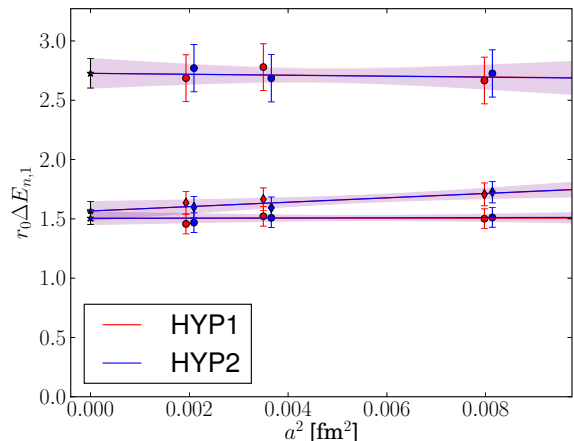
Figure 15: Continuum limits (stars) of \Delta E_{n,1}^{\text{stat}} (circles) and \Delta E_{2,1}^{\text{HQET}} (diamonds). Shown are the results for both HYP1 (red, shifted to the left) and HYP2 (blue, shifted to the right). Graph from [121].
