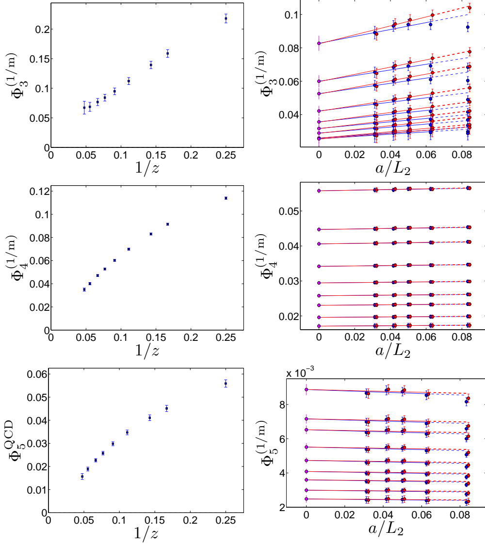
Figure 9: \Phi_i^{(1/m_h)}(L_1) = \Phi_i^{\text{QCD}}(L_1) - \eta_i(L_1) , i = 3, 4 in L_1 on the left and their step scaling function to obtain \Phi_i^{(1/m_h)}(L_2) = \Phi_i^{\text{QCD}}(L_2) - \eta_i(L_2) on the right. The bottom line shows \Phi_5(L_1) ; spin symmetry means that its static part vanishes, \eta_5 = 0 . The b-quark in Nature has about 1/z \approx 0.08 .
