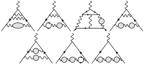
Figure 2: Diagrams contributing to the hadronic vacuum polarization at next-to-next-to-leading order.
