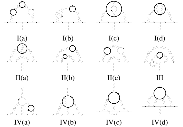
Figure 1: Classes of diagrams considered in Ref. [12]. Thin and thick lines denote light and heavy leptons, respectively.
