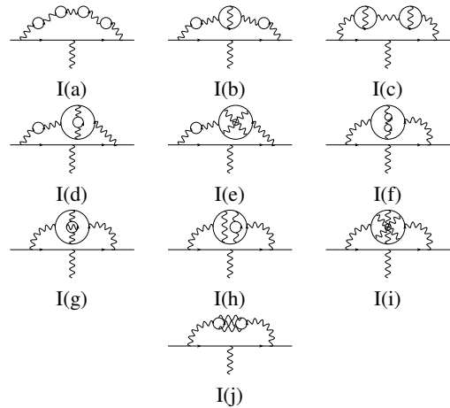
Figure 3: Diagram classes considered in the analysis of Ref. [17].
