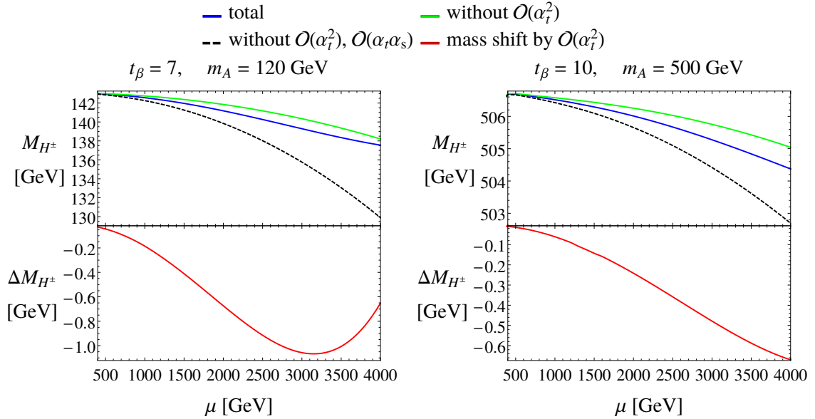
Figure 4. Upper parts: prediction for the charged Higgs-boson mass M_{H^\pm} including all known contributions (blue), without the \mathcal{O}(\alpha_t^2) contributions (green) and without any two-loop corrections (black dashed). Lower parts: the mass shift \Delta M_{H^\pm} by the \mathcal{O}(\alpha_t^2) contributions (red). Left: t_\beta = 7 , m_A = 120 GeV, A_t = A_b = A_\tau = 2.5 m_{\tilde{q}_3} . Right: t_\beta = 10 , m_A = 500 GeV, A_t = A_b = A_\tau = 1.5 m_{\tilde{q}_3} . The other input parameters are m_{\tilde{q}_3} = m_{\tilde{t}_R} = m_{\tilde{b}_R} = 1000 GeV, m_{\tilde{t}_3} = m_{\tilde{\tau}_R} = 1000 GeV, m_{\tilde{g}} = 1500 GeV, for both cases.
