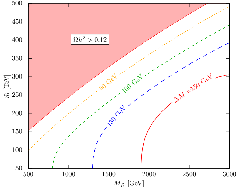
Figure 2: Contour for the mass difference \Delta M which makes the thermal relic abundance of bino DM equal to the observed DM density \Omega_{\text{DM}} h^2 = 0.12 . In the red shaded region the bino DM is overproduced due to failure of bino-gluino coannihilation.
