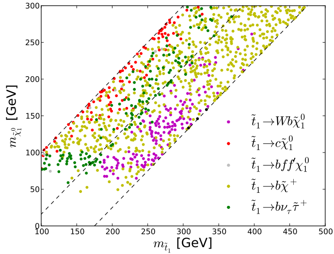
Figure 7. Scatter plot in the (m_{\tilde{t}_1}, m_{\tilde{\chi}_1^0}) plane of the \tilde{t}_1 decay modes with branching ratios > 50\% for 1000 randomly-selected points with m_{\tilde{t}_1} - m_{\tilde{\chi}_1^0} < m_t .
