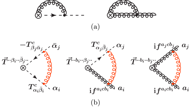
FIG. 1. (a) Collinear one-loop diagrams. (b) Soft one-loop diagrams connecting two fields i and j in the operator.
