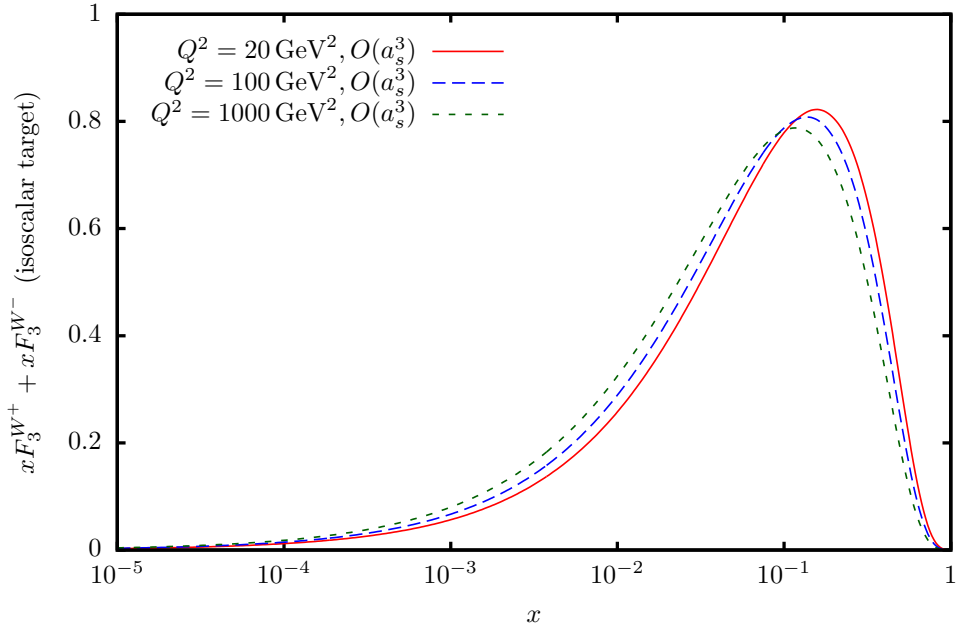
Figure 5: The corrections up to 3-loop order to the combination of the structure functions xF_3^{W^+}(x, Q^2) + xF_3^{W^-}(x, Q^2) off a nucleon in an isoscalar target, including both the massless and charm contributions in the asymptotic approximation.
