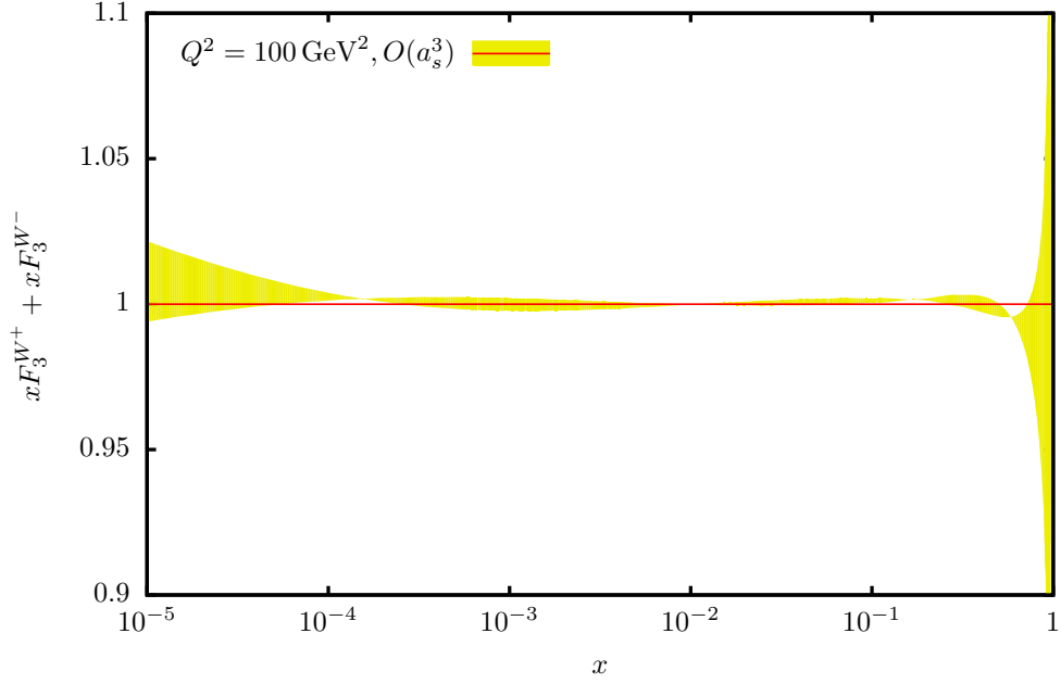
Figure 4: The ratio of the structure functions xF_3^{W^+}(x, \mu^2) + xF_3^{W^-}(x, \mu^2) to xF_3^{W^+}(x, Q^2) + xF_3^{W^-}(x, Q^2) , varying \mu^2 \in [Q^2/4, 4Q^2] at O(a_s^3) and Q^2 = 100 \text{ GeV}^2 as a function of x .
