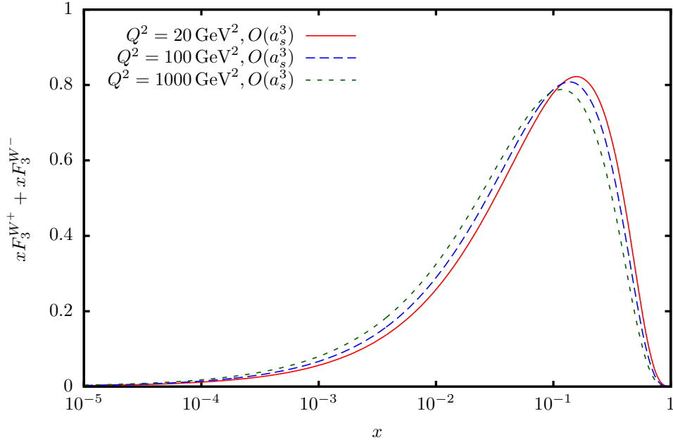
Figure 1: The corrections up to 3-loop order to the combination of the structure functions xF_3^{W^+}(x, Q^2) + xF_3^{W^-}(x, Q^2) off a proton target, including both the massless and the charm contributions in the asymptotic approximation in the on-shell scheme for m_c = 1.59 GeV [17] as a function of x and Q^2 . The parton distribution functions of Ref. [52] have been used with \alpha_s(M_Z^2) = 0.1132 . These settings are the same in the subsequent Figures.
