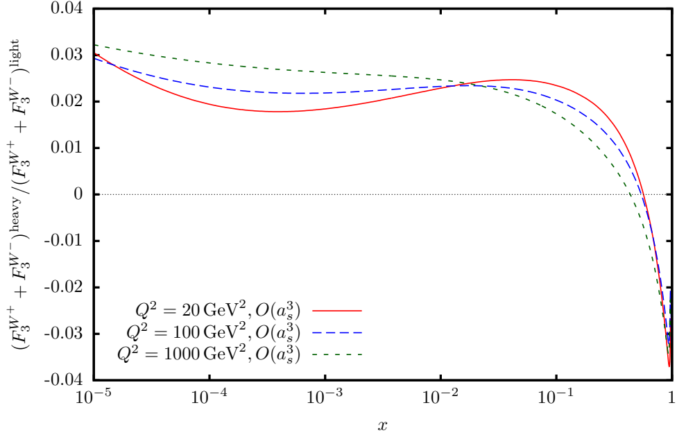
Figure 2: Ratio of the structure functions x F_3^{W^+}(x, Q^2) + x F_3^{W^-}(x, Q^2) off a proton target up to 3-loop order for the charm contribution and the massless terms for three flavors.
