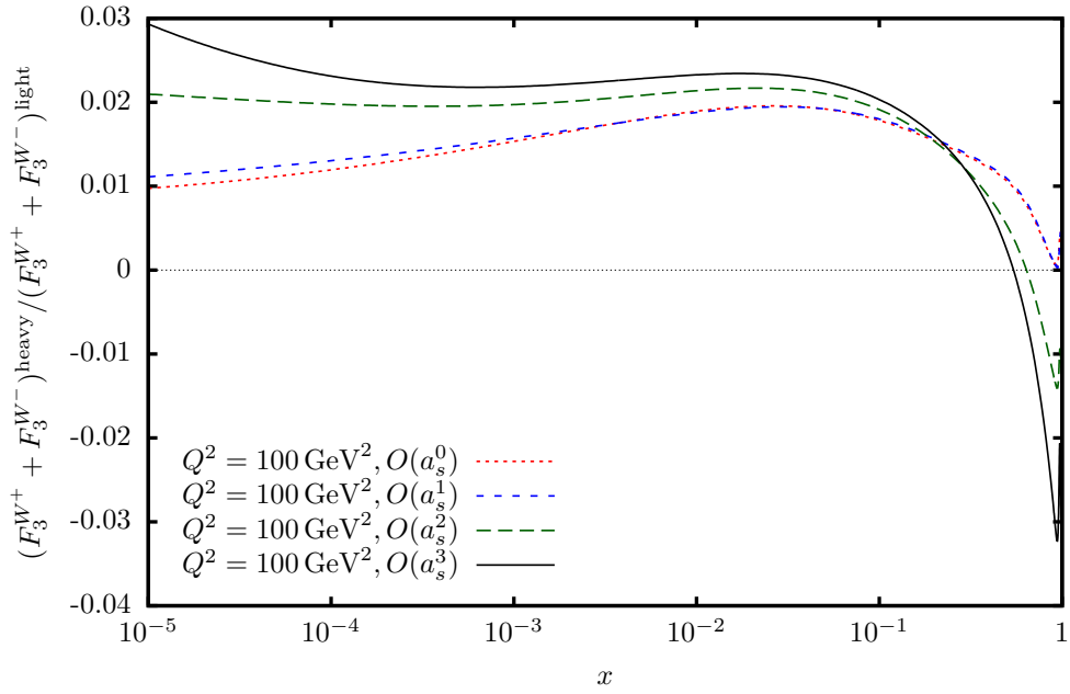
Figure 3: Ratio of the structure functions x F_3^{W^+}(x, Q^2) + x F_3^{W^-}(x, Q^2) off a proton target up to 3-loop order for the charm contribution and the massless terms for three flavors from tree-level to O(a_s^3) at Q^2 = 100 \text{ GeV}^2 .
