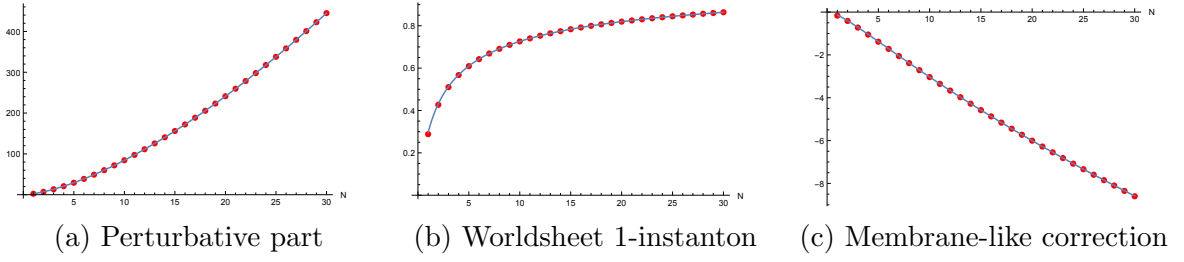
Figure 8. We show the plot of resummed free energy S_0 F of ABJM theory as a function of N for k = 17/5 . The solid curves represent some combinations of Airy functions computed from J_{\text{Borel}}(\mu) while the red dots are the numerical values of S_0 F . More precisely, each figure represent: (a) the (minus of) free energy -S_0 F and the perturbative free energy -\log Z_{\text{pert}} . (b) The worldsheet 1-instanton normalized by the exponential factor e^{2\pi\sqrt{2\lambda}} : (e^{S_0 F}/Z_{\text{pert}} - 1)e^{2\pi\sqrt{2\lambda}} and Z_{\text{WS}}^{(1)}e^{2\pi\sqrt{2\lambda}} . (c) The membrane-like correction normalized by the exponential factor e^{k\pi\sqrt{2\lambda}} : (e^{S_0 F}/Z_{\text{pert}} - 1 - Z_{\text{WS}}^{(1)})e^{k\pi\sqrt{2\lambda}} and Z_{\text{np}}^{(1)}e^{k\pi\sqrt{2\lambda}} .
