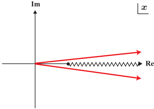
Figure 7. When t is real, the integrand in (1.2) has a branch cut along x \geq |t/g_s| . One has to deform the integration contour in order to avoid this branch cut. As shown by the red arrows, there are two such deformations, and these two lead to different lateral resummations (5.15).
