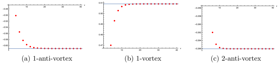
Figure 2. We show the plots of F_{\text{vor}}^{\text{resum}}(b, v) as a function of v for b = 6/5 . The solid lines represent the expected vortex or anti-vortex coefficients, while the red dots represent the numerical values of the integral (3.7). More precisely, the red dots in each figure represent: (a) F_{\text{vor}}^{\text{resum}}(b, v)e^{v/b} , (b) [F_{\text{vor}}^{\text{resum}}(b, v) - F_{\text{vor}}^{(1)}(b, v)]e^{bv} , (c) [F_{\text{vor}}^{\text{resum}}(b, v) - F_{\text{vor}}^{(1)}(b, v) - F_{\text{vor}}^{(2)}(b, v)]e^{2v/b} . Here F_{\text{vor}}^{(\ell)} (or F_{\text{vor}}^{(\ell)}(b, v) ) denotes the \ell -vortex (or \ell -anti-vortex) contribution, respectively.
