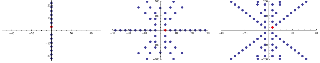
Figure 6. We show the singularities of \mathcal{B}[\tilde{F}_{\text{coni}}^{\text{GV}}](\zeta) in the Borel plane for t = \frac{i}{2} (Left), t = \frac{1}{2} (Middle) and t = \frac{1}{2} + \pi i (Right). For t \in \mathbb{R} , there exist an infinite number of singularities on the positive real axis, and thus the genus expansion is non-Borel summable. For t \in \mathbb{R} + \pi i , on the other hand, no singularities lie on the positive real axis. In all the cases, one of the closest singularities to the origin is located at \zeta = 2\pi t , which we show by the red points.
