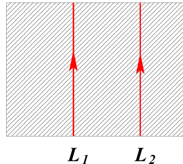
Figure 4: In the presence of surface operator and/or Omega-background line operators do not commute.
