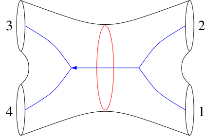
Figure 5: Pants decomposition of four-holed sphere with a numbering of boundary components.
