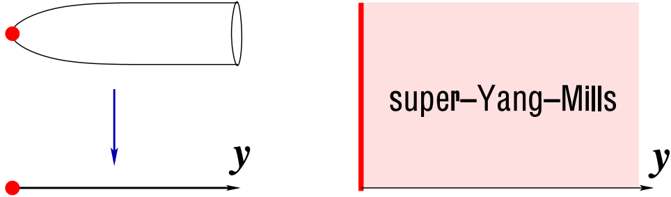
Figure 3: The six-dimensional (2, 0) theory with a codimension-2 defect at the tip of the cigar reduces to 5d super-Yang-Mills theory with a non-trivial boundary condition.
