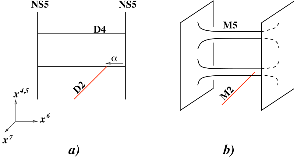
Figure 2: The brane construction of a surface operator in pure \mathcal{N} = 2 super Yang-Mills theory (a) in type IIA string theory and (b) its M-theory lift.
