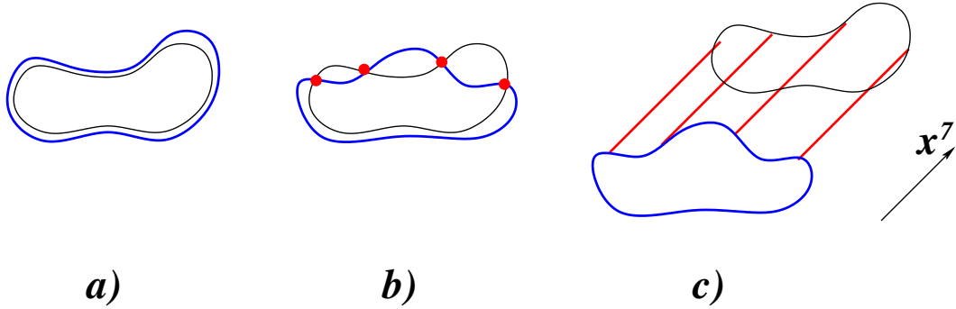
Figure 1: An M5'-brane wrapped on the curve C can be perturbed to a curve \tilde{C} which meets C at finitely many points u_i . Then, separating the five-branes on C and \tilde{C} along the x^7 direction results in creation of M2-branes (shown in red).
