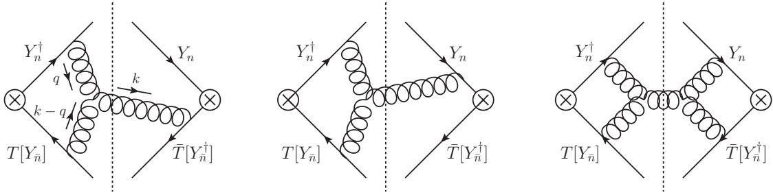
Figure 6. Diagrams contribution to H_s for e^+e^- \rightarrow 3 jets. The left and middle diagram are the nonvanishing contributions to S^{(1,0)} . The right diagram gives S^{(1,1)} , entering H_s at two loops.
