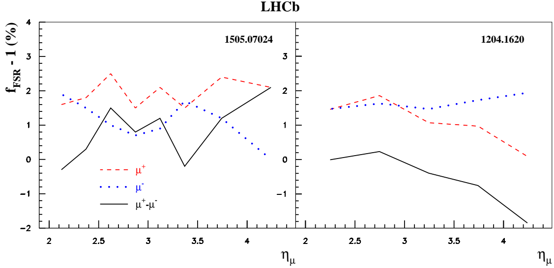
FIG. 5: Left panel: Correction for the final-state-radiation (FSR) effects applied in the LHCb analysis [18] to the data on the pseudo-rapidity distribution of muons produced in forward W^{\pm} -decays (dashes: \mu^+ , dots: \mu^- , solid: difference between these two). Right panel: The same for the earlier LHCb analysis of Ref. [21].
