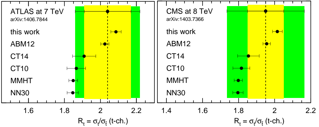
FIG. 13: Same as in Fig. 11 for the ratio of cross sections R_t = \sigma_t/\sigma_{\bar{t}} in comparison to ATLAS data [15] at \sqrt{s} = 7 TeV (left) and to CMS data [16] at \sqrt{s} = 8 TeV (right).
