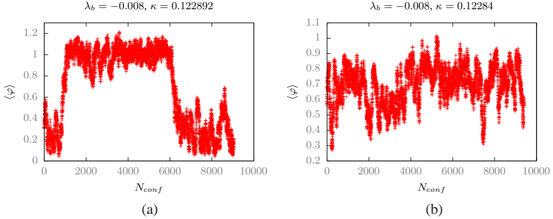
Figure 3: The Monte-Carlo time evolution of \langle\varphi\rangle near phase transitions at (a) \kappa = 0.122892 and the lattice volume 20^3 \times 4 , (b) \kappa = 0.12284 and the lattice volume 20^3 \times 6 .
