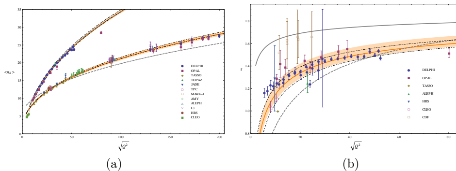
Fig. 3. Comparisons of fit results for (a) \langle n_h(Q^2) \rangle_g , \langle n_h(Q^2) \rangle_q , and (b) r(Q^2) with experimental data. 73 The experimental and theoretical uncertainties are indicated by the shaded/orange bands and the bands enclosed between the dot-dashed curves, respectively.
