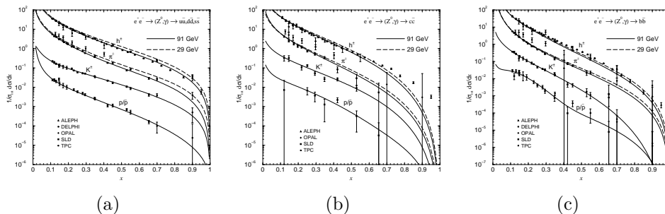
Fig. 1. Comparisons of the cross sections of process (1) for h = h^\pm, \pi^\pm, K^\pm, p/\bar{p} with (a) a = u, d, s , (b) a = c , and (c) a = b evaluated using the fitted FFs with the experimental data sets included in the fit 46,46–52 and one by OPAL 54 without hadron identification. 38 The theoretical results for h = h^\pm are taken to be the sums of the respective ones for h = \pi^\pm, K^\pm, p/\bar{p} . The theoretical results for a = g are distributed among the respective ones for a = u, d, s, c, b according to the flavor of the q\bar{q} pair produced along with the gluon.
