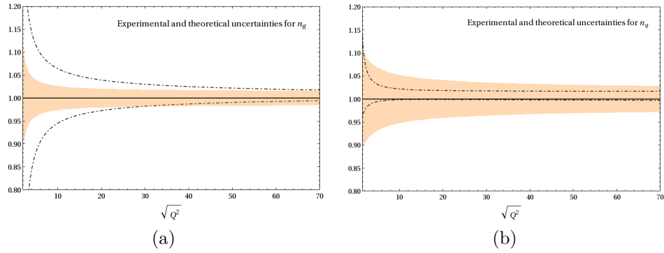
Fig. 4. Experimental (shaded/orange bands) and theoretical (bands enclosed between dot-dashed curves) uncertainties in the N^3\text{LO}_{\text{approx}}+\text{NLO}+\text{NNLL} results for (a) \langle n_h(Q^2) \rangle_g and (b) \langle n_h(Q^2) \rangle_q normalized with respect to their default evaluations. 73
