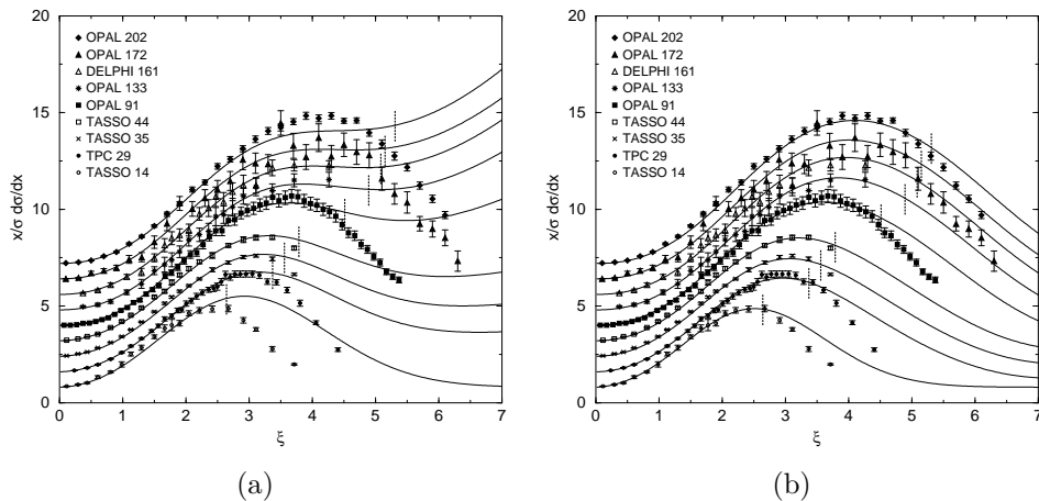
Fig. 2. LO fits to small- x data of process (1) (a) without and (b) with resummation of double logarithms. 60
