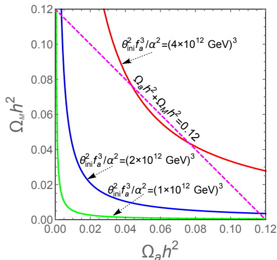
FIG. 1. Relation between the axion and monopole abundances. We take \theta_{\text{ini}}^2 f_a^3 / \alpha^2 = (10^{12} \text{ GeV})^3 (green curve), (2 \times 10^{12} \text{ GeV})^3 (blue curve), and (4 \times 10^{12} \text{ GeV})^3 (red curve). The diagonal (magenta) dashed line represents the observed DM abundance.
