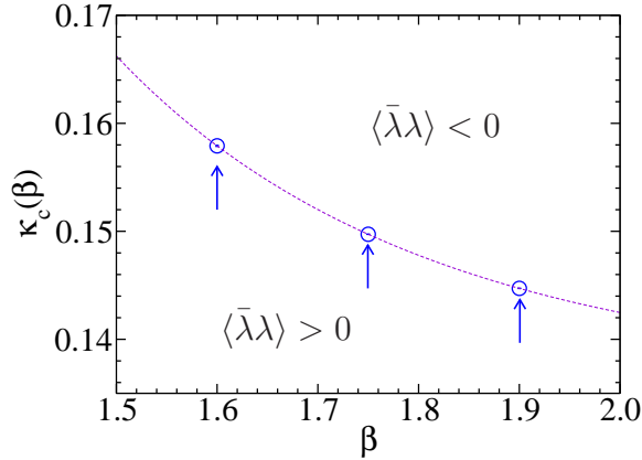
Figure 1: Masses of particles are first extrapolated to the chiral limit, i.e. to the critical value of \kappa where the gluino mass vanishes, and then to the continuum limit, \beta \rightarrow \infty . The critical line \kappa_c(\beta) separates the bare parameter space into two regions characterised by either a positive or a negative expectation value of the gluino condensate. Chiral extrapolations at \beta = 1.6 and \beta = 1.75 have been presented in Ref. [8] and Ref. [10, 12], respectively.
