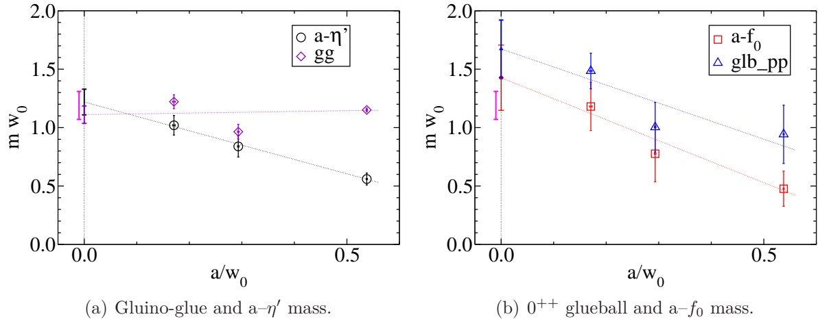
Figure 4: a) Extrapolations of the a\text{-}\eta' and gluino-gluon masses to the continuum limit. The large gap visible at the largest lattice spacing is drastically reduced at larger \beta . b) Extrapolations of the a\text{-}f_0 and 0^{++} glueball masses to the continuum limit. The extrapolation of the glueball mass is unstable and dominated by the result at small lattice spacing, therefore the final result is compatible with the gluino-gluon mass only within two standard deviations. The thick vertical magenta line represents the weighted mean value of the four masses.
