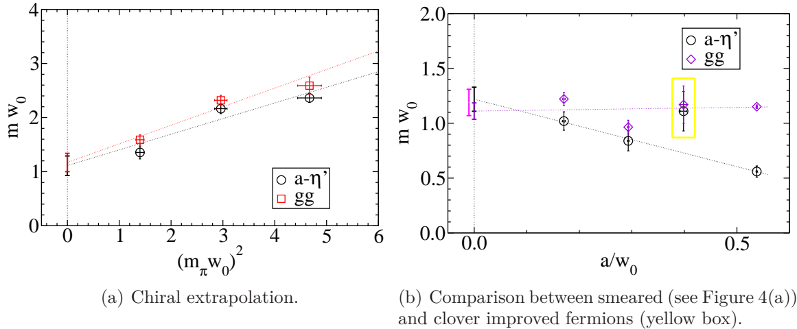
Figure 6: a) Extrapolation of the a\text{-}\eta' and gluino-gluon masses to the chiral limit computed with tadpole improved clover fermions. b) Comparison of the extrapolations to the continuum limit of the a\text{-}\eta' and gluino gluon masses with the tadpole clover improved action results (yellow box). Despite the large lattice spacing, the results obtained with the improved action are in agreement with the continuum limit extrapolation using the action with one level of stout smearing on the fermions.
