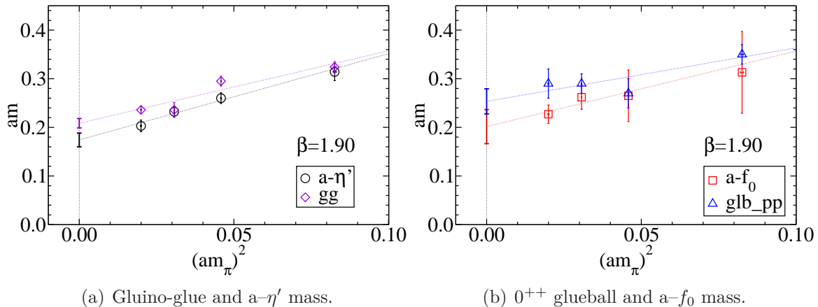
Figure 3: Extrapolation to the chiral limit at \beta = 1.90 .
