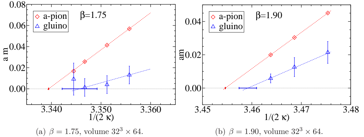
Figure 2: Comparison between the values of \kappa_c defined as the value of \kappa where the square of the a- \pi mass or the renormalised gluino mass am_S Z_S^{-1} vanishes. The horizontal thick lines (red and blue) show the uncertainty in the determination of the intercept with zero.
