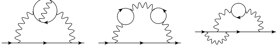
Figure 3: Propagator type diagrams with electron loops contributing to the mass and field renormalization constants. The middle diagram can contain two electron loops or one electron and one muon loop.
