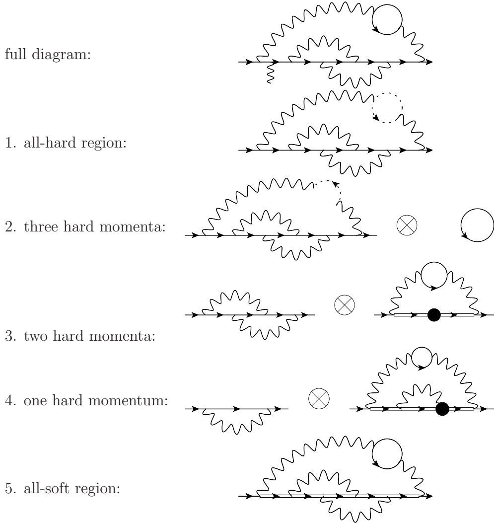
Figure 2: Relevant regions of an example Feynman diagram with an electron loop. The first line contains the full diagram and in rows two to six one representative sub-diagram for each region is shown. The dotted lines denote massless (electron) propagators, the solid lines massive (muon or electron) propagators and the solid double lines represent linear propagators of the form 1/(2\ell \cdot q) where q is the external momentum with q^2 = m_\mu^2 and \ell is a loop momentum.
