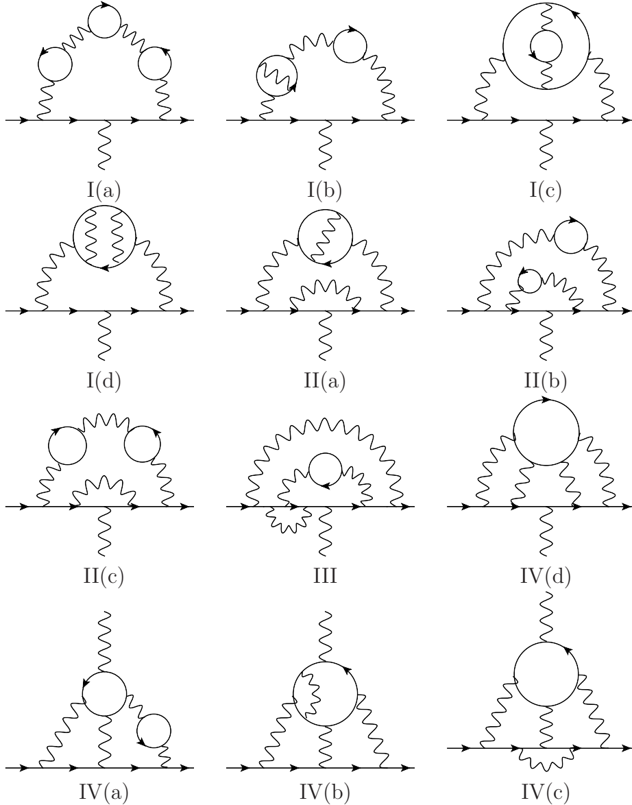
Figure 1: Four-loop example Feynman diagrams contributing to a_\mu containing at least one closed electron loop. The external solid lines represent muons, the solid loops denote electrons, muons or taus, and the wavy lines represent photons.
