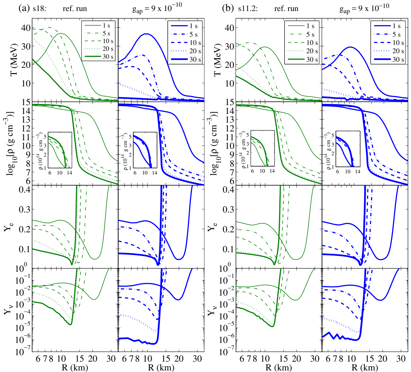
FIG. 5: (color online) Evolution of selected quantities – from top to bottom: temperature, density, electron and neutrino abundances – during the PNS deleptonization, comparing our reference simulations (left panels) with the simulation including axions (right panels) with ( g_{\text{ap}} = 9 \times 10^{-10} , \xi = 1 ).
