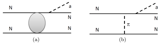
FIG. 1: Example diagrams for the axion production through N – N axion bremsstrahlung ( N = neutron or proton). The shaded region in 1(a) represents bulk nuclear interactions and 1(b) shows the contribution of the OPE approximation.
