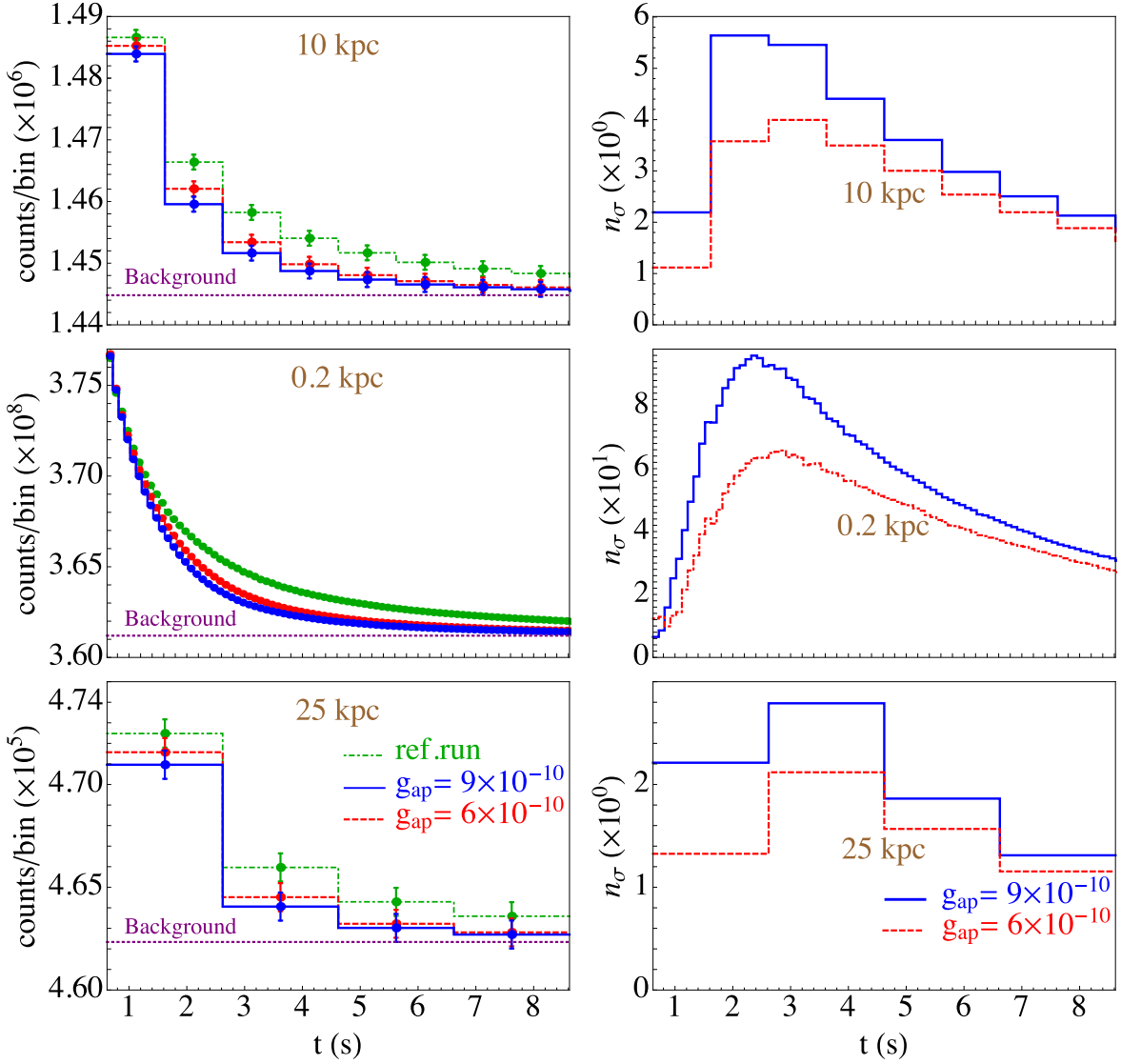
FIG. 13: (color online) Same as Fig. 11 but for the IceCube detector.
