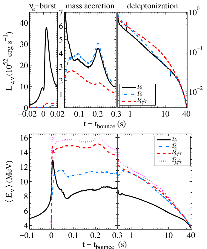
FIG. 2: (color online) Evolution of neutrino energy luminosities (top panel) and average energies (bottom panel) for the reference simulation of s18.
