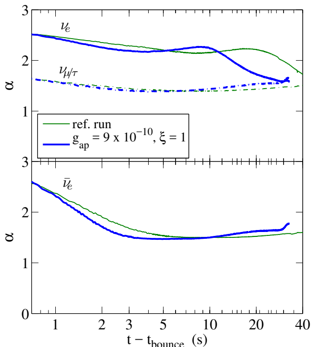
FIG. 9: (color online) Dimensionless energy-shape parameter Eq. (16) for s18 comparing the reference case without axions and the simulation with axions ( g_{\text{ap}} = 9 \times 10^{-10} , \xi = 1 ).
