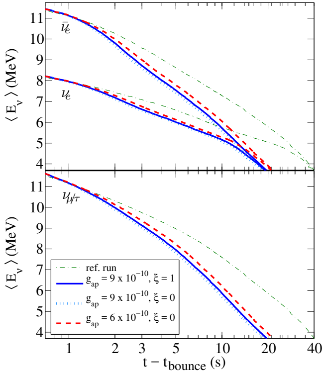
(b) Average neutrino energies
