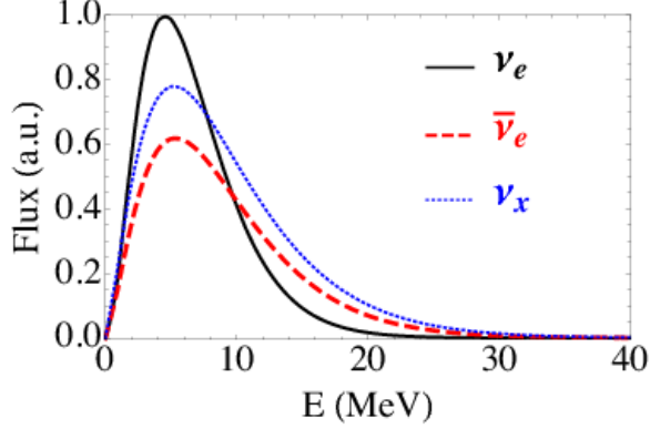
(b) Ref. case ( g_{\text{ap}} = 0 ) – PNS deleptonization phase
