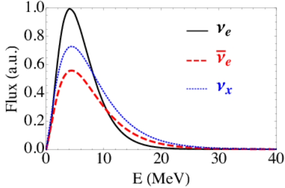
(c) ( g_{\text{ap}} = 9 \times 10^{-10}, \xi = 1 ) – PNS deleptonization phase
