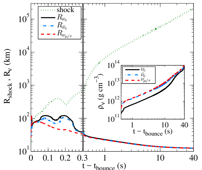
FIG. 3: (color online) Evolution of shock radius and neutrinospheres for the reference simulation of s18. The inlay shows the density at the corresponding neutrinospheres.
