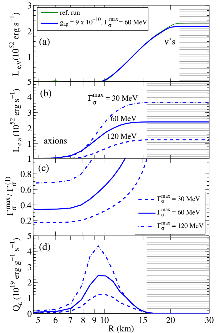
FIG. 4: (color online) Radial profiles of selected quantities at 1 s post bounce (see text for definitions).
