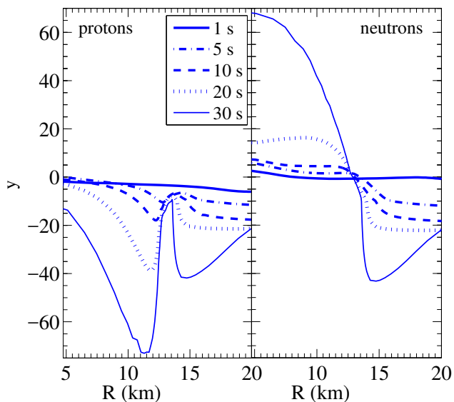
FIG. 8: (color online) Degeneracy for protons ( left panel ) and neutrons ( right panel ) for the simulation with axions ( g_{\text{ap}} = 9 \times 10^{-10} , \xi = 1 ) at selected post bounce times corresponding to the PNS profiles illustrated in the right panel of Fig. 5 (a).
