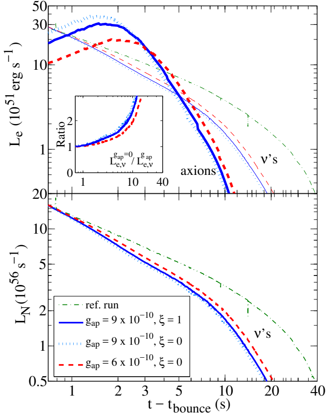
(a) Energy and number luminosities
