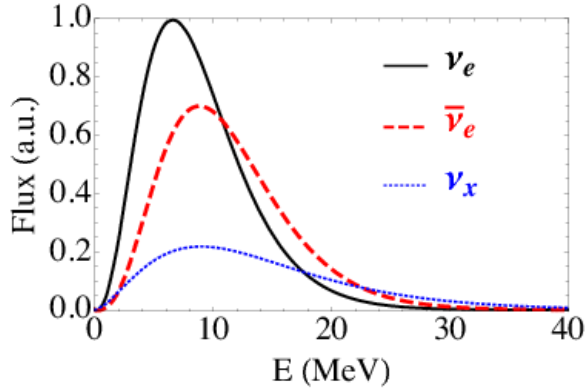
(a) Ref. case ( g_{\text{ap}} = 0 ) – mass accretion phase
