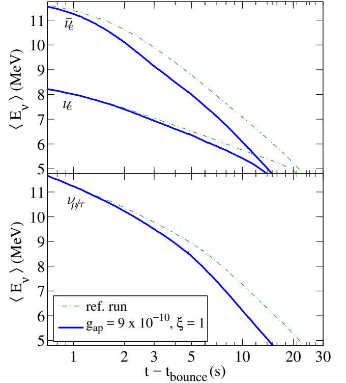
(b) Average neutrino energies
