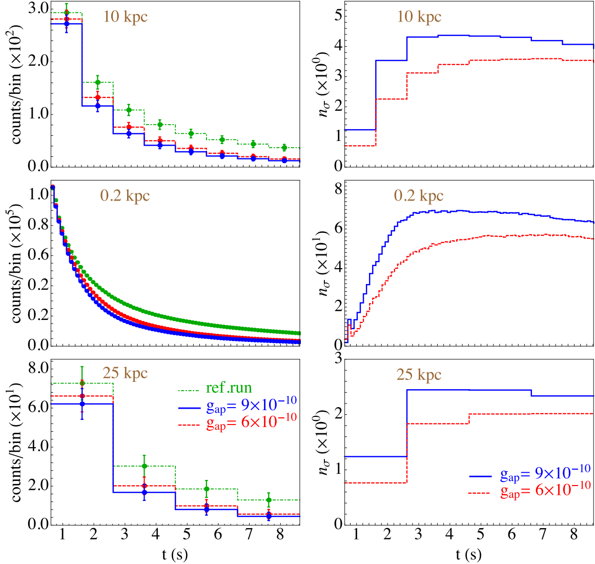
FIG. 11: (color online) Left panel: Super-Kamiokande neutrino event rate based on s18 at selected SN distance – 10 kpc (top panel), 0.2 kpc (middle panel) and 25 kpc (bottom panel) – comparing the reference model and simulations with axions included ( g_{\text{ap}} = 9 \times 10^{-10} , \xi = 1 ) and ( g_{\text{ap}} = 6 \times 10^{-10} , \xi = 0 ). Right panel: Corresponding ratios relative to the reference case.
