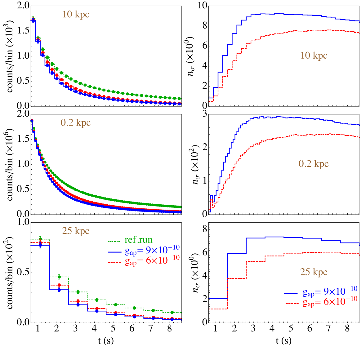
FIG. 12: (color online) Same as Fig. 11 but for the 400 kton Water Cherenkov detector.
