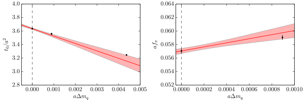
Figure 2: Examples of the mass shifts for the t_0 and f_\pi along the symmetric line m_{\text{ud}} = m_s at \beta = 3.46 . The data points correspond to the measurements on the ensembles H400, H401 and H402. The shaded bands give the linear approximation to the mass dependence starting from the leftmost point. Deviations from the linear approximation are smaller than the increase in the statistical uncertainties.
