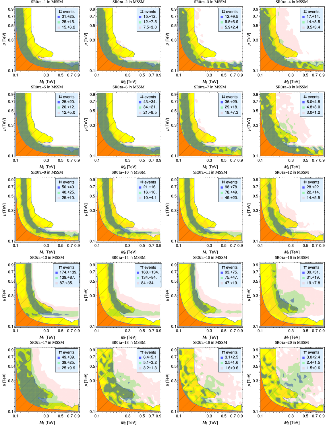
Figure 6. Three-lepton search - MSSM - 13 TeV: Number of events in the SR0 \tau of the three-lepton search in the \{\mu, M_2\} -plane for the MSSM. From left to right and top to bottom we show the 20 bins as labelled. The blue region denotes the number of signal events in the SR in between the maximum and its 80%. The green (pink) regions indicate the number of signal events in between the 50% (20%) and 80% (50%) of its maximum. In yellow we show the region excluded by Run 1, while in orange we denote the excluded region for charginos from LEP.
