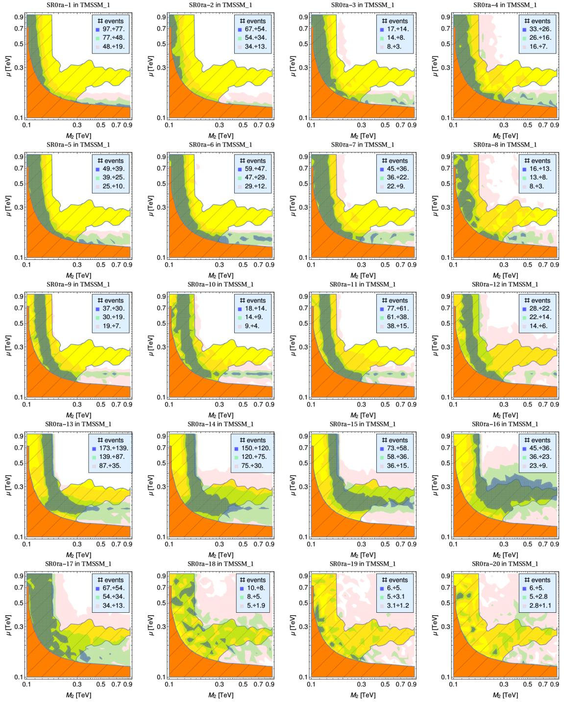
Figure 8. Three-lepton search - TMSSM_1 - 13 TeV: Same as Fig. 6 for the TMSSM_1 case ( \lambda = 0.65 and \mu_\Sigma = 300 GeV).
