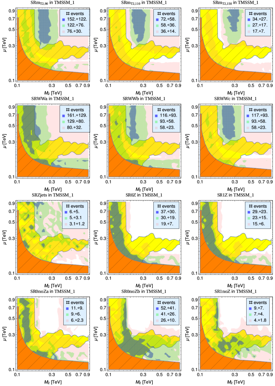
Figure 7. Two-lepton & four-lepton searches - TMSSM_1 - 13 TeV: Same as Fig. 5 for the TMSSM_1 case ( \lambda = 0.65 and \mu_\Sigma = 300 GeV).
