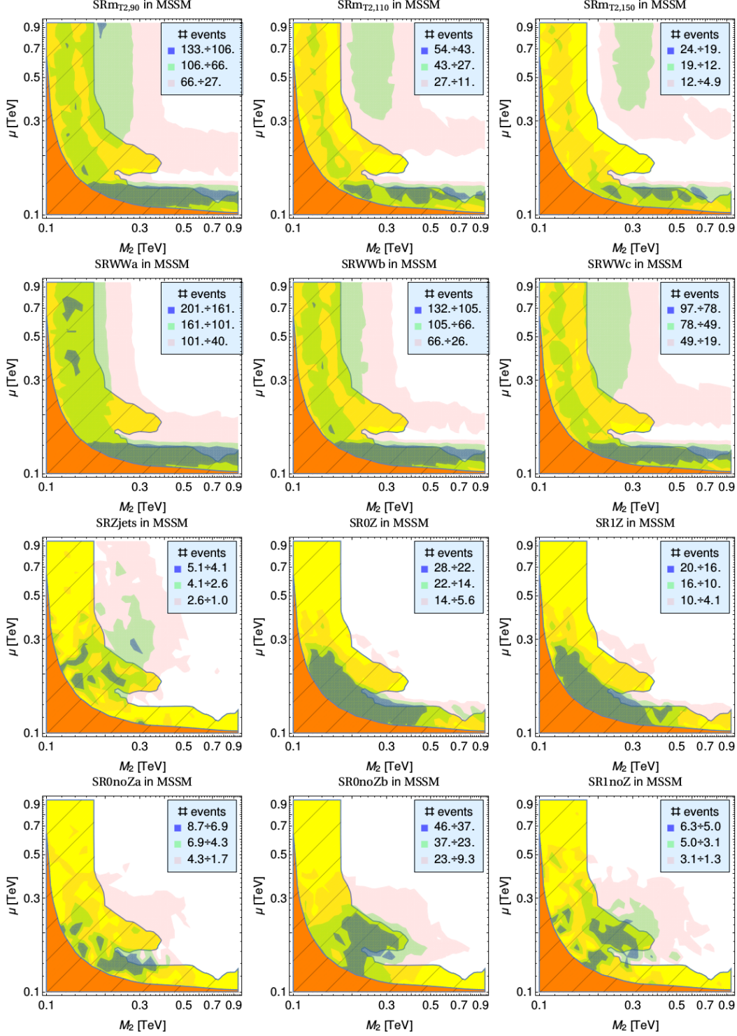
Figure 5. Two-lepton & four-lepton searches - MSSM - 13 TeV: Number of events in the two-lepton and four-lepton search SRs in the \{\mu, M_2\} -plane for the MSSM. From left to right and top to bottom for the two-lepton + MET: SRm T_{2,90} , SRm T_{2,110} , SRm T_{2,150} , SRWWa, SRWWb, SRWWc and SRZjets, as labelled. For the four-lepton case from left to right and top to bottom following the two-lepton SRs: SR0Z, SR1Z, SR0noZa, SR0noZb and SR1noZ. The blue region denotes the number of signal events in the SR in between the maximum and its 80%. The green (pink) regions indicate the number of signal events in between the 50% (20%) and 80% (50%) of its maximum. In yellow we show the region excluded by Run 1, while in orange we denote the excluded region for charginos from LEP.
