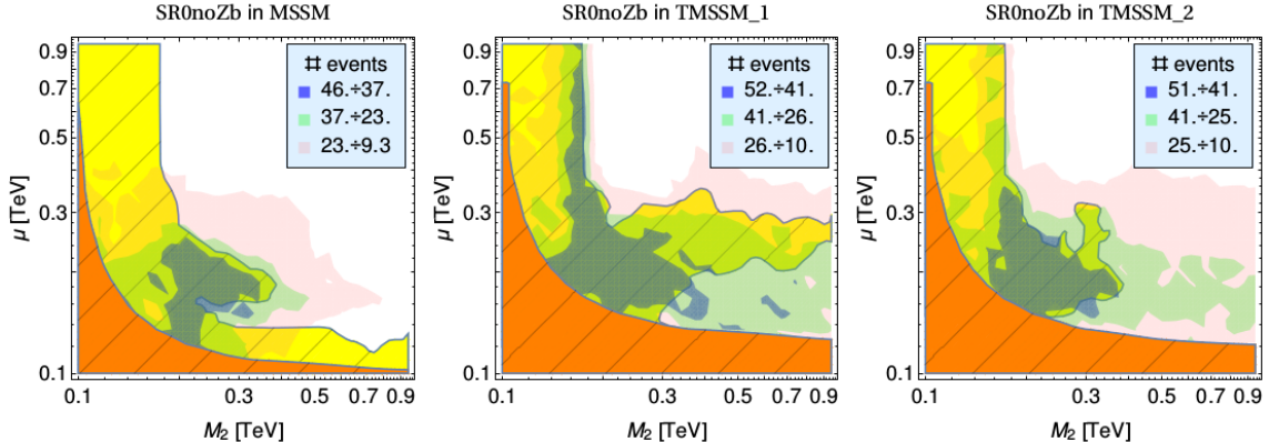
Figure 3. Same as Fig. 2 but for the SRnoZb region of the four-lepton analysis.
