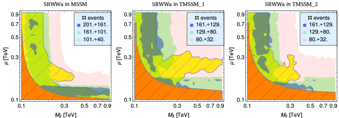
Figure 2. Number of expected signal events, as labelled, in the MSSM (left panel), the TMSSM_1 (center panel) and the TMSSM_2 (right panel) in the SRWWa region of the two-lepton analysis. The excluded regions (yellow and orange for the LHC Run 1 bound and chargino mass bound respectively), surrounded by the solid line, are over-imposed.
