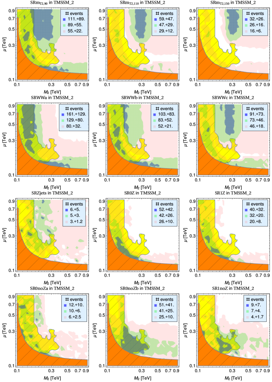
Figure 9. Two-lepton & four-lepton searches - TMSSM 2 - 13 TeV: Same as Fig. 5 for the TMSSM 2 case ( \lambda = 0.65 and \mu_\Sigma = 350 GeV).
