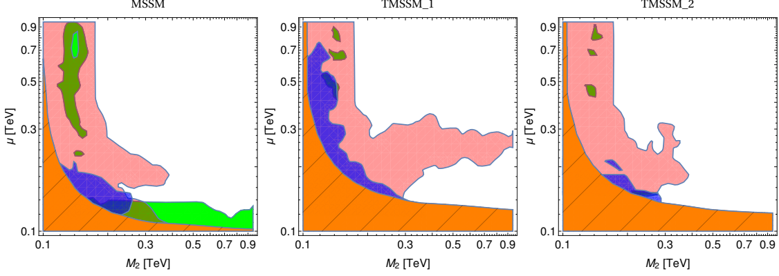
Figure 1. Left: Excluded regions at 95% CL after the LHC Run 1 for the MSSM scenario with \tan\beta = 10 . The green, pink and blue shaded regions are the excluded regions from the two-lepton, three-lepton and four-lepton + MET search respectively, while the shaded orange region denotes the LEP bound on the chargino mass at 95% CL. Other panels: Same as left for the TMSSM.1 ( \lambda = 0.65 , \mu_\Sigma = 300 GeV, \tan\beta = 3 ) and TMSSM.2 ( \lambda = 0.65 , \mu_\Sigma = 350 GeV, \tan\beta = 3 ) scenarios in the central and right panel respectively. In all panels the lightest neutralino is fixed at m_{\tilde{\chi}_1^0} = 63 GeV.
