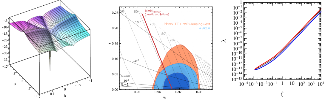
Figure 1: Left: Decadic log of the SMASH scalar potential in the Einstein frame, as a function of Higgs in the unitary gauge, h , and the modulus of \sigma , \rho , all in units of M_P , for \kappa_H < 0 , \kappa_\sigma < 0 , supporting mixed Higgs-Hidden-Scalar Inflation along one of the valleys. Middle: Bounds on r vs. n_s [18], compared to the predictions from (H)HSI in SMASH for fixed values of the non-minimal coupling \xi_\sigma and the number of e-folds N , respectively. Right: Required self-coupling versus non-minimal coupling to reproduce CMB results on inflation. All figures from [11].
