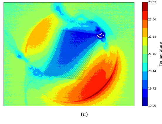
Figure 13: Temperature maps of the silicon side of the micro-channel wafer taken with an infrared camera with the heater set to 30.8 \text{ mW cm}^{-2} and the superimposed channel structure. (a) 10 \text{ ml min}^{-1} , (b) 30 \text{ ml min}^{-1} , (c) 50 \text{ ml min}^{-1} .
