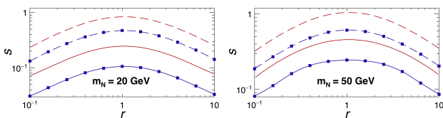
FIG. 6. Discovery and exclusion limits for Majorana sterile neutrinos with m_N = 20 (left) and 50 (right) GeV. The blue curves marked with squares correspond to 3- \sigma limit, while the red curves correspond to 5- \sigma limit; solid lines for BDT method and dashed lines for CC method.
