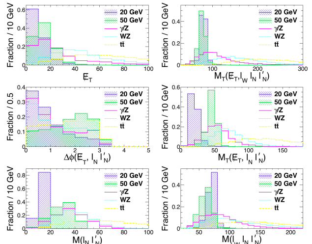
FIG. 3. Kinematical distributions for Dirac signals with m_N = 20 and 50 GeV, and SM backgrounds of \gamma^*/Z +jets, WZ +jets and t\bar{t} +jets after applying the basic cuts and b-jets veto.
