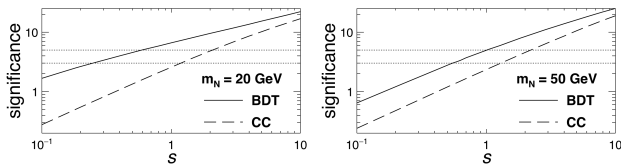
FIG. 5. Discovery and exclusion limits for Dirac sterile neutrinos with m_N = 20 (left) and 50 (right) GeV.
