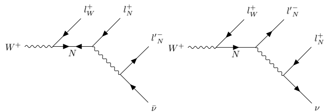
FIG. 1. Left: LNV process W^+ \rightarrow l_W^+ l_N^+ l_N'^- \bar{\nu} , mediated by a heavy sterile neutrino of Majorana type only. Right: the LNC process W^+ \rightarrow l_W^+ l_N^- l_N^+ \nu , mediated by a heavy sterile neutrino of either Majorana or Dirac type.
