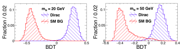
FIG. 4. Distributions of BDT response for Dirac signal (blue) with m_N = 20 (left) and 50 (right) GeV, and total SM backgrounds (red) including \gamma^*/Z +jets, WZ+jets and t\bar{t} +jets.
