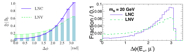
FIG. 7. The \Delta\phi(\mathcal{E}_T, \mu^-) distributions in the N rest frame from the W^+ \rightarrow e^+e^+\mu^-\nu process for the benchmark point m_N = 20 GeV by theoretical calculation (left) and data simulation (right). Solid blue and dashed green lines correspond to LNC and LNV processes, respectively.
