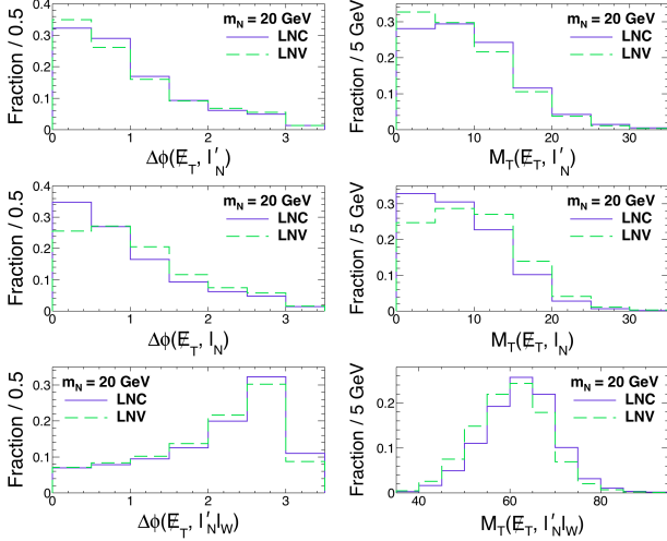
FIG. 8. Distributions for the benchmark point m_N = 20 GeV after applying the basic cuts, b-jet vetoes and the first BDT cut.
