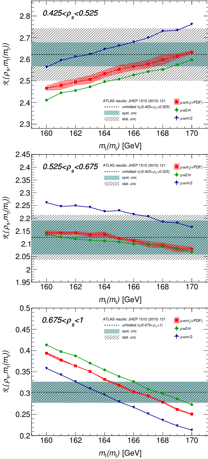
Fig. 3. \mathcal{R} as defined in Eq. (3) as a function of m_t(m_t) for \rho_s > 0.425 intervals.
