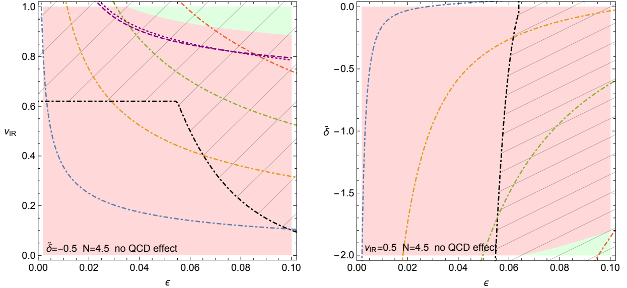
Figure 4: Results for \mu_{\min} = 2.5 TeV and N = 4.5 without the QCD effect. For the left panel, we have fixed \tilde{\delta} = -0.5 , and for the right panel, v_{\text{IR}} = 0.5 . Regions where the phase transition can complete via the nucleation of O(4) -symmetric bubbles are shown in green, while regions where the nucleation rate is too low are colored in red. Regions above the purple dashed and dotted lines are allowed according to the analytical estimate of the bubble action for O(4) - and O(3) -symmetric bubbles, respectively. In the hashed region (above the black, dashed line in the left panel and to right of the black, dashed line in the right panel), the backreaction constraint is not fulfilled. The blue, orange, green, red dashed-dotted lines (from bottom to top in the left panel and in the reversed order in the right panel) correspond to the radion mass being m_{\text{radion}} = 200 GeV, 600 GeV, 1 TeV, 1.4 TeV, respectively.
