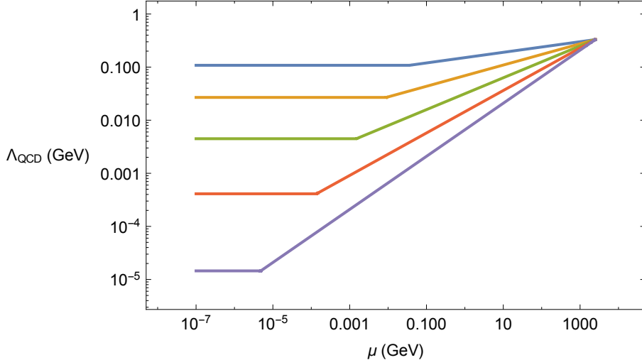
Figure 1: Schematic plot of the QCD confinement scale \Lambda_{\text{QCD}} as a function of the IR scale \mu for \mu_{\text{min}} = 2.5 \text{ TeV} , n_c = 3 and n = 0.1, 0.2, 0.3, 0.4, 0.5 (in blue, yellow, green, red, purple).
