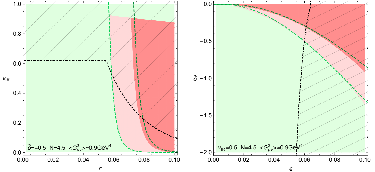
Figure 5: Results for \mu_{\text{min}} = 2.5 \text{ TeV} , N = 4.5 and n = 0.1 and n = 0.3 when the QCD effect is included. For the left panel, we have fixed \tilde{\delta} = -0.5 , and for the right panel, v_{\text{IR}} = 0.5 . Regions where the phase transition can complete via the nucleation of O(4) -symmetric bubbles for both n = 0.1 and n = 0.3 are shown in green. This to be compared with the allowed regions in fig. 4 without the QCD effect. Regions where the nucleation rate is too low are colored in pale (dark) red for n = 0.3 ( n = 0.1 ). The corresponding green dashed lines delimit the region satisfying eq. (6.5), where we expect the QCD effect to be important. In the hashed region (above the black, dashed line in the left panel and to right of the black, dashed line in the right panel), the backreaction constraint is not fulfilled. The radion masses are as in fig. 4.
