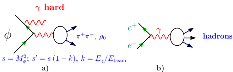
Figure 6. a) Initial state radiation (ISR) on resonance, b) Standard energy scan by tuning the beam energy.
