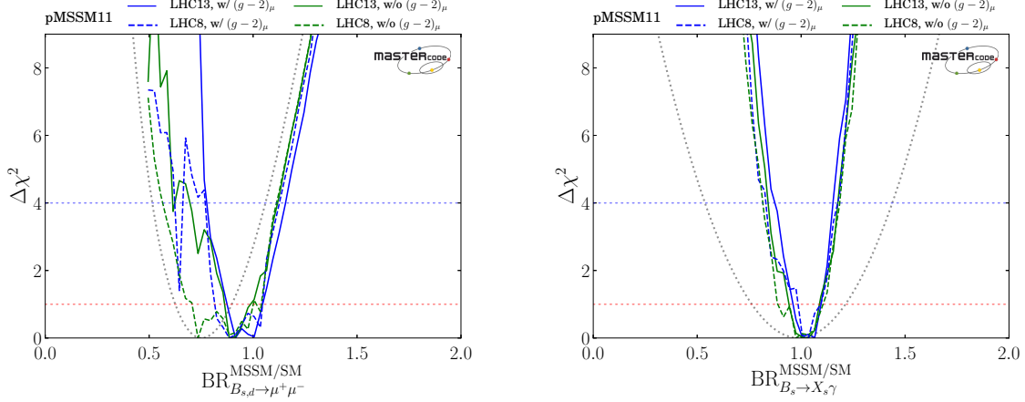
Figure 14. One-dimensional profile likelihood functions for \text{BR}(B_{s,d} \rightarrow \mu^+ \mu^-) in the pMSSM11 (left panel) and the \text{BR}(B_s \rightarrow X_s \gamma) branching ratio (right panel), with and without the LHC 13-TeV data and the (g-2)_\mu constraint. Also shown as dotted lines are the experimental constraints, including the corresponding theoretical uncertainties within the Standard Model.
