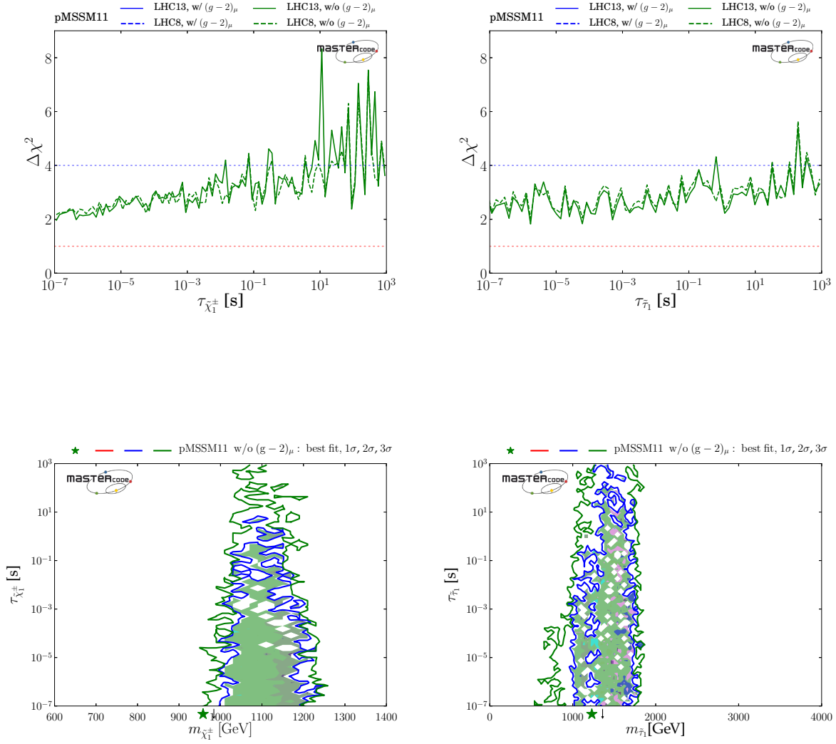
Figure 19. Upper panels: one-dimensional profile likelihood plots for the lifetime of the \tilde{\chi}_1^\pm (left) and the \tilde{\tau}_1 (right). Lower panels: the corresponding mass-lifetime planes for the \tilde{\chi}_1^\pm and \tilde{\tau}_1 , with the 95% CL regions shaded according to the dominant DM mechanisms.
