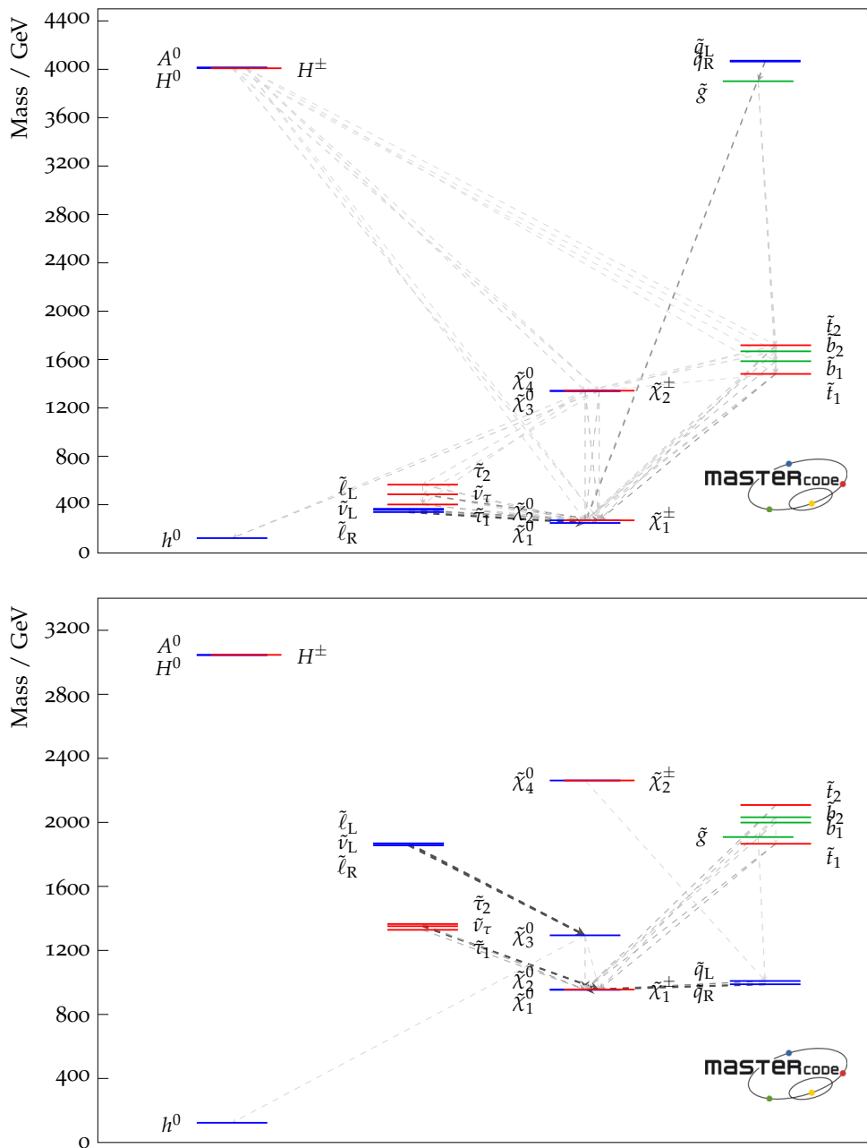
Figure 1. Higgs and sparticle spectra for the best-fit points for the pMSSM11 with (top) and without the (g-2)_\mu constraint (bottom), showing also decay paths with branching ratios > 5\% , the widths of the lines being proportional to the branching ratios. These plots were prepared using the code presented in [86].
