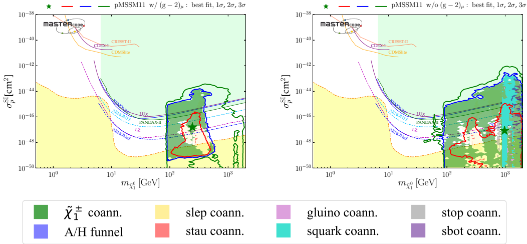
Figure 20. Planes of (m_{\tilde{\chi}_1^0}, \sigma_p^{\text{SI}}) with (left panel) and without (right panel) the (g-2)_\mu constraint applied, where the values of \sigma_p^{\text{SI}} displayed are the nominal values calculated using the SSARD code. The upper limits established by the LUX [4], XENON1T [6] and PandaX-II [3] Collaborations are shown as green, magenta and blue contours, respectively, and the combined limit is indicated by a black line with green shading above. The projected future 90% CL exclusion sensitivities of the LUX-Zeplin (LZ) [91] and XENON1T/nT [92] experiments are shown as solid purple and dashed blue lines, respectively, and the neutrino background ‘floor’ is shown as a dashed orange line with yellow shading below.
