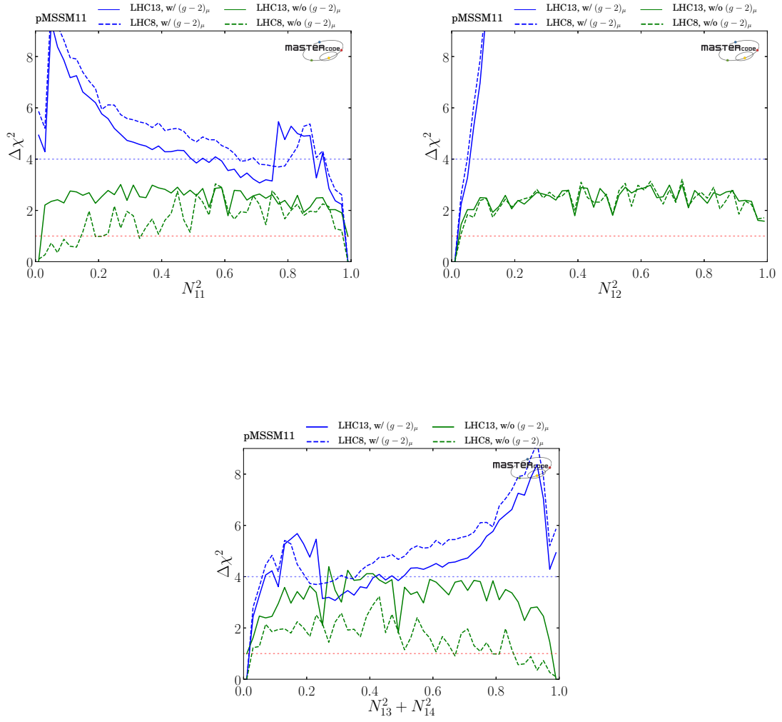
Figure 12. One-dimensional likelihood plots for the \tilde{B} fraction in the LSP \tilde{\chi}_1^0 composition in the (upper left), for the \tilde{W}^3 fraction (upper right) and for the \tilde{H}_{u,d} fraction (lower panel).
