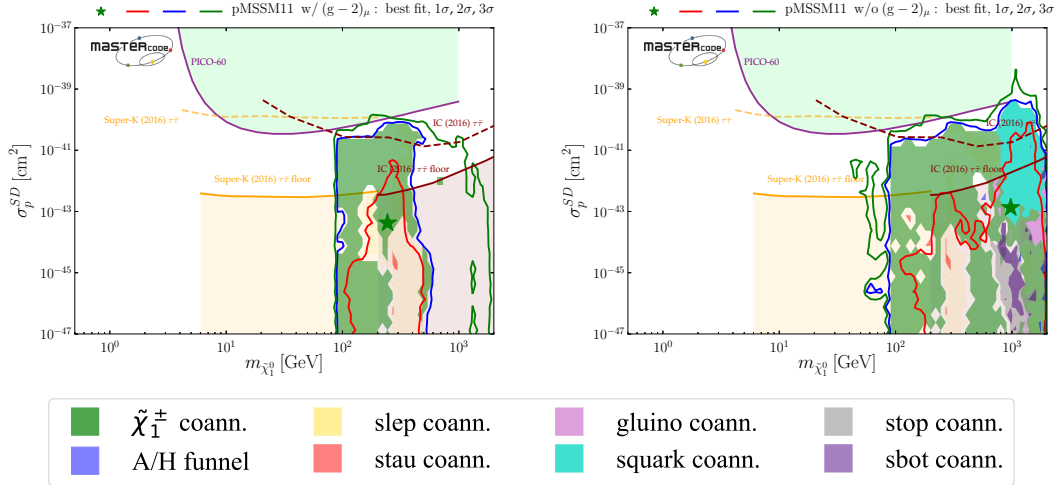
Figure 21. Planes of (m_{\tilde{\chi}_1^0}, \sigma_p^{SD}) with (left panel) and without (right panel) the (g-2)_\mu constraint applied, where the values of \sigma_p^{SD} displayed are the nominal values calculated using the SSARD code [37]. The upper limit established by the PICO Collaboration [5] is shown as a purple contour, with green shading above. The neutrino ‘floor’ for \sigma_p^{SD} is taken from [93]. We also show the indicative upper limits from SuperKamiokande [94] and IceCube [75] searches for energetic solar neutrinos obtained assuming that the LSPs annihilate predominantly into \tau^+\tau^- , which are subject to the caveats discussed in the text.
