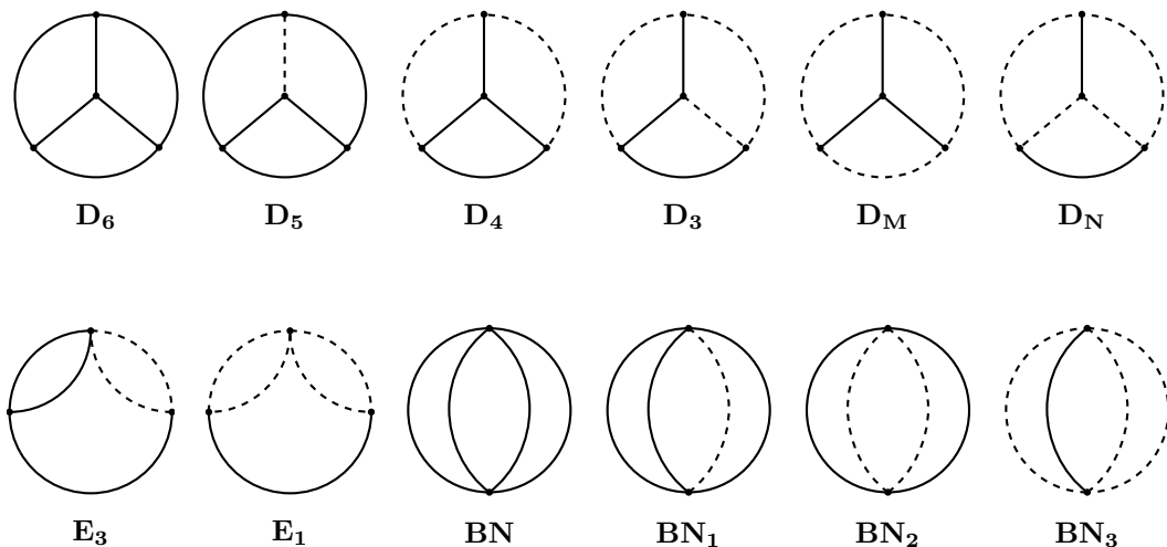
Figure 1. Full set of non-factorizing master integrals. Solid and dashed lines correspond to massive and massless scalar propagators, respectively.
