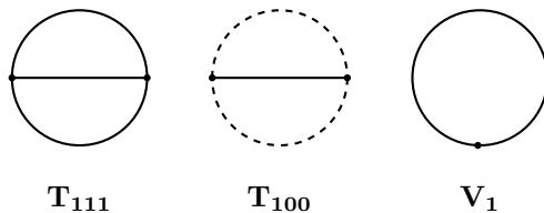
Figure 2. Two-loop and one-loop master integrals. The line coding is the same as in figure 1.
