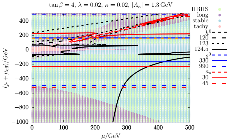
Figure 12: Vacuum stability analysis for a scenario with small value of \lambda , but potentially large values of \tilde{\kappa} along the diagonal line of \mu_{\text{eff}} \approx 0 \text{ GeV} . The masses of the SM-like Higgs boson and the singlet-like \mathcal{CP} -even and -odd states are indicated in black, blue and red, respectively. The green area is allowed by HiggsBounds and HiggsSignals ; with the gray band, the direct exclusion bound on light charginos is shown. Superimposed with orange dashes is the line of constant \mu + \mu_{\text{eff}} = 160 \text{ GeV} , along which Figs. 9–11 are defined.
