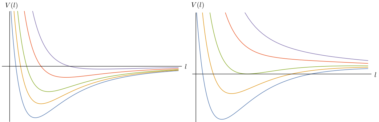
Figure 1: Left: Off-shell potential V(l) for the S^2 volume modulus in the case without a 6D c.c. for n = 25 flux units and different values of the dimensionless three-brane tension \mathcal{T}_3 : \mathcal{T}_3 = 0 in blue, \mathcal{T}_3 = 0.1 in yellow, \mathcal{T}_3 = 0.21 in green, \mathcal{T}_3 = 0.4 in red and \mathcal{T}_3 = 0.6 in purple. As can be seen, the more energy density, the higher the vacuum energy, but the flattening prevents the minimum to go above zero. Right: Off-shell potential V(l) for the S^2 volume modulus in the case with a 6D c.c. for n = 25 flux units, \mathcal{T}_5 = 0.004 and different values of the dimensionless three-brane tension \mathcal{T}_3 : \mathcal{T}_3 = 0 in blue, \mathcal{T}_3 = 0.1 in yellow, \mathcal{T}_3 = 0.21 in green, \mathcal{T}_3 = 0.4 in red and \mathcal{T}_3 = 0.6 in purple. This time it is also possible to find the Sitter minima once enough three-brane tension has been added.
