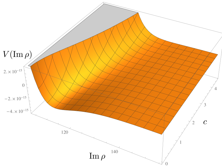
Figure 4: The F-term potential of (17) for the case b = 0 as a function of the uplift parameter c . In this case the superpotential reads W = W_0 + A(1 + cS)\exp(ia\rho) . The \rho -minimum moves out to larger values and stays AdS as c increases. This behavior is compatible with our 10D analysis but does not uniquely follow from it.
