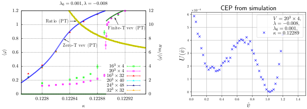
Figure 1. Results for \lambda_6 = 0.001 and \lambda = -0.008 . In the left-hand panel, the errors are statistical from lattice computations, and symbols without errors represent results obtained in perturbative calculations using the constraint effective potential. “Ratio” means \langle\varphi\rangle/m_H , and “PT” stands for “perturbation theory”. In this figure, the Higgs vev, \langle\varphi\rangle , is plotted in lattice units. The right-hand side is the constraint effective potential, obtained in the Monte-Carlo simulation at non-zero temperature, and at the four-volume (L/a)^3 \times (T/a) = 20^3 \times 4 and \kappa = 0.12289 .
