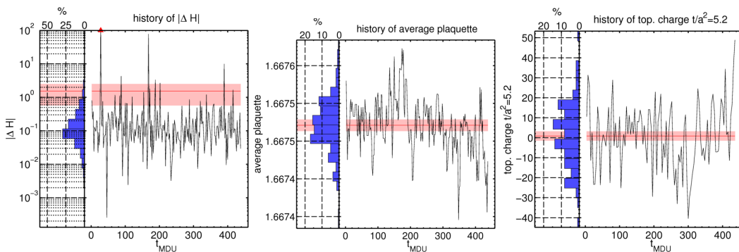
Figure 6: Left pane: MD history of \Delta H for the physical mass run E250. Mid pane: MD history of the average plaquette. Right pane: History of the topological charge at the center of the lattice.
